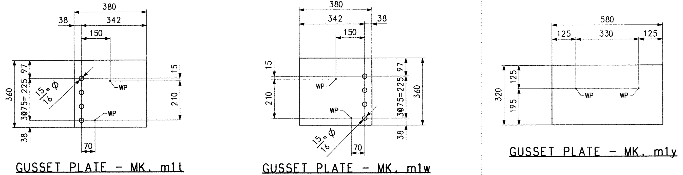
GUSSET PLATE - MK.m1m (CG) GUSSET PLATE - MK.m1n (CG) GUSSET PLATE - MK.m1p GUSSET PLATE - MK.m1s
