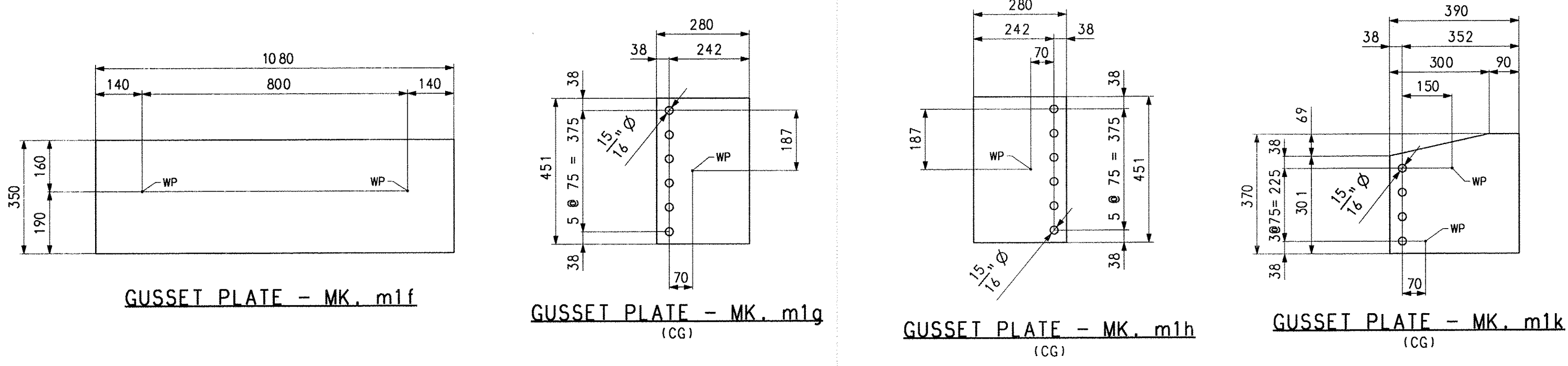
GUSSET PLATE - MK.m1a GUSSET PLATE - MK.m1b GUSSET PLATE - MK.m1c GUSSET PLATE - MK.m1d
