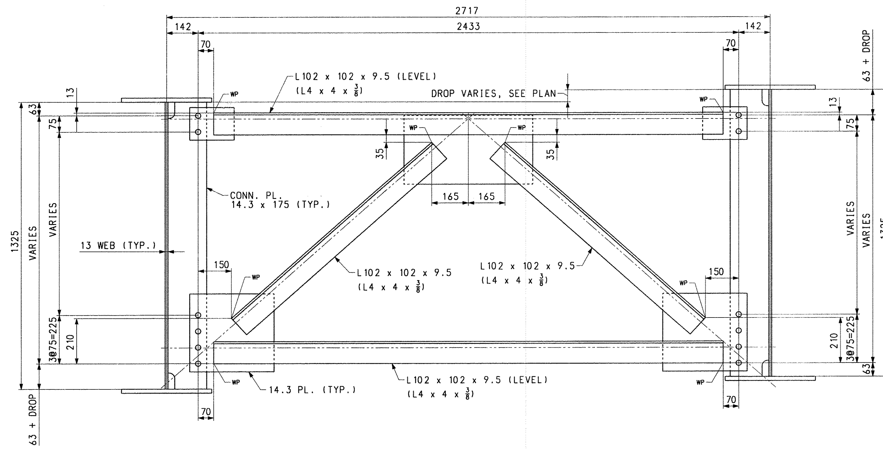
TYP. INT. CROSSFRAME LAYOUT (LOOKING BACKSTATIONS)
