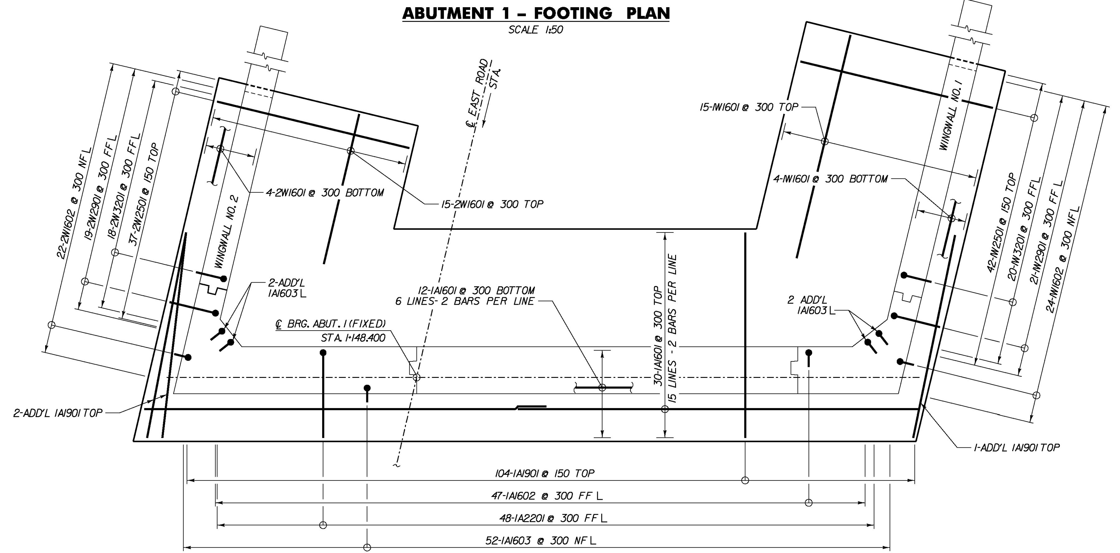
ABUTMENT 1 - FOOTING REINFORCEMENT PLAN SCALE 1:50
