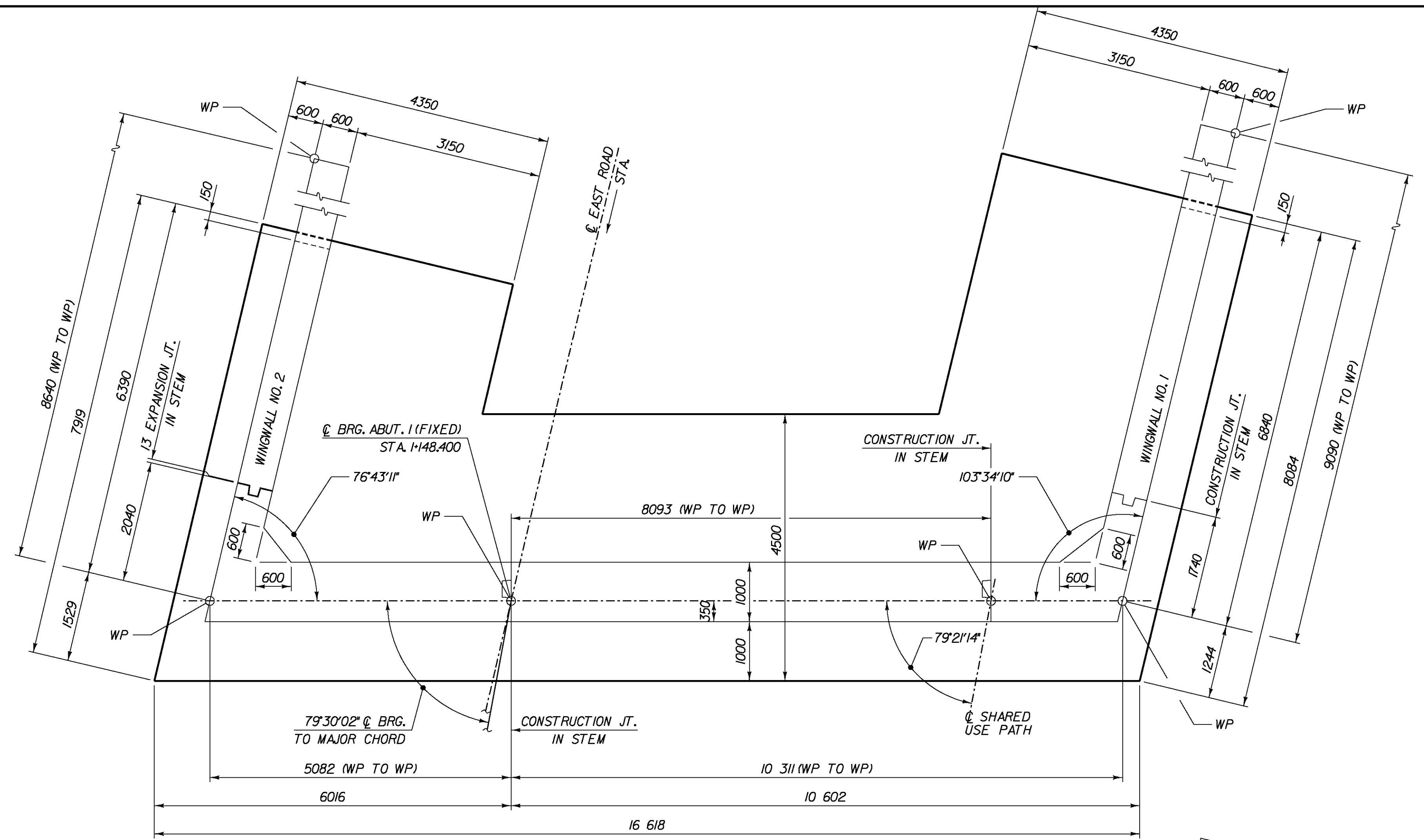
ABUTMENT 1 - FOOTING PLAN SCALE 1:50
