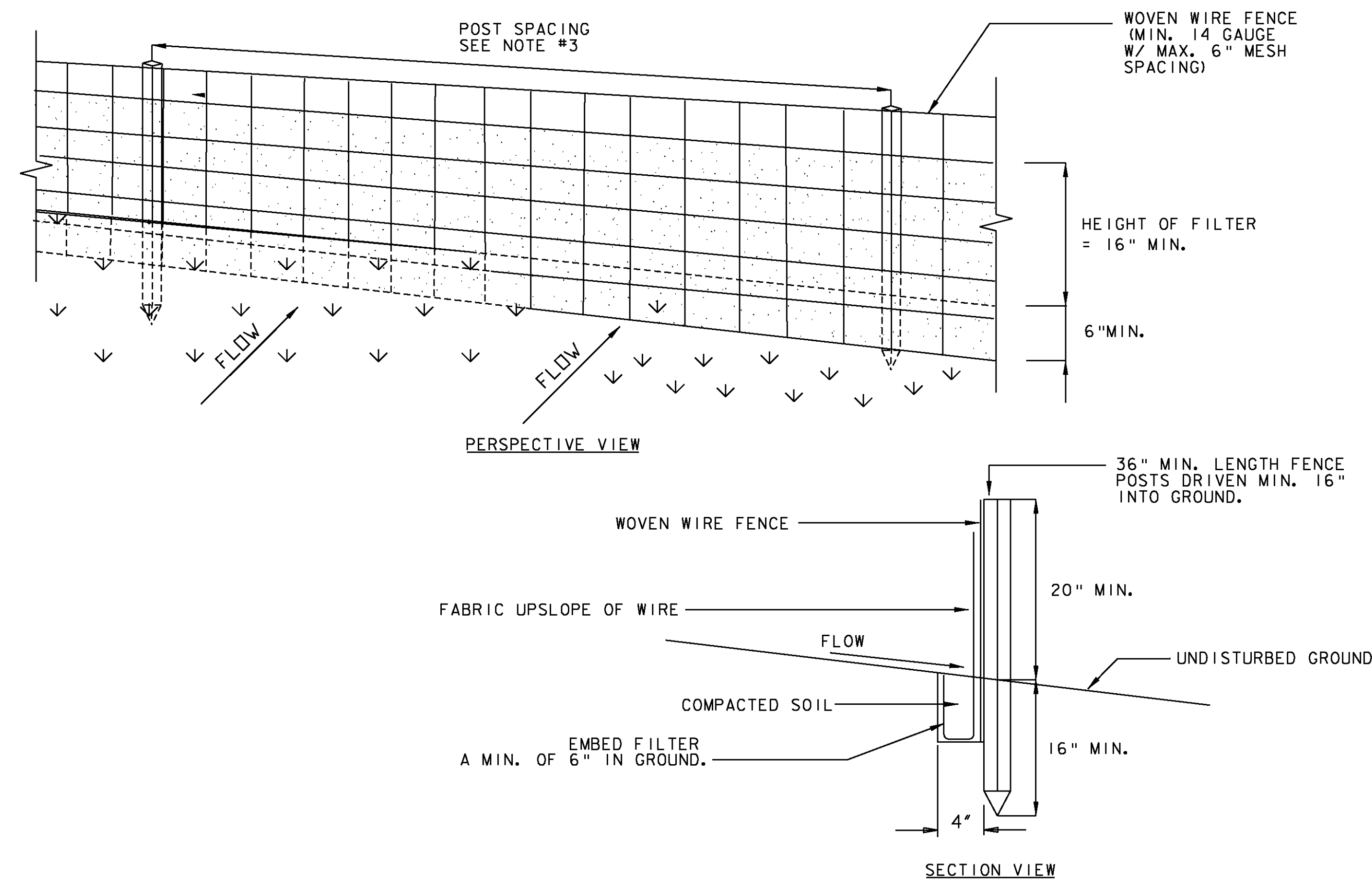
SILT FENCE
