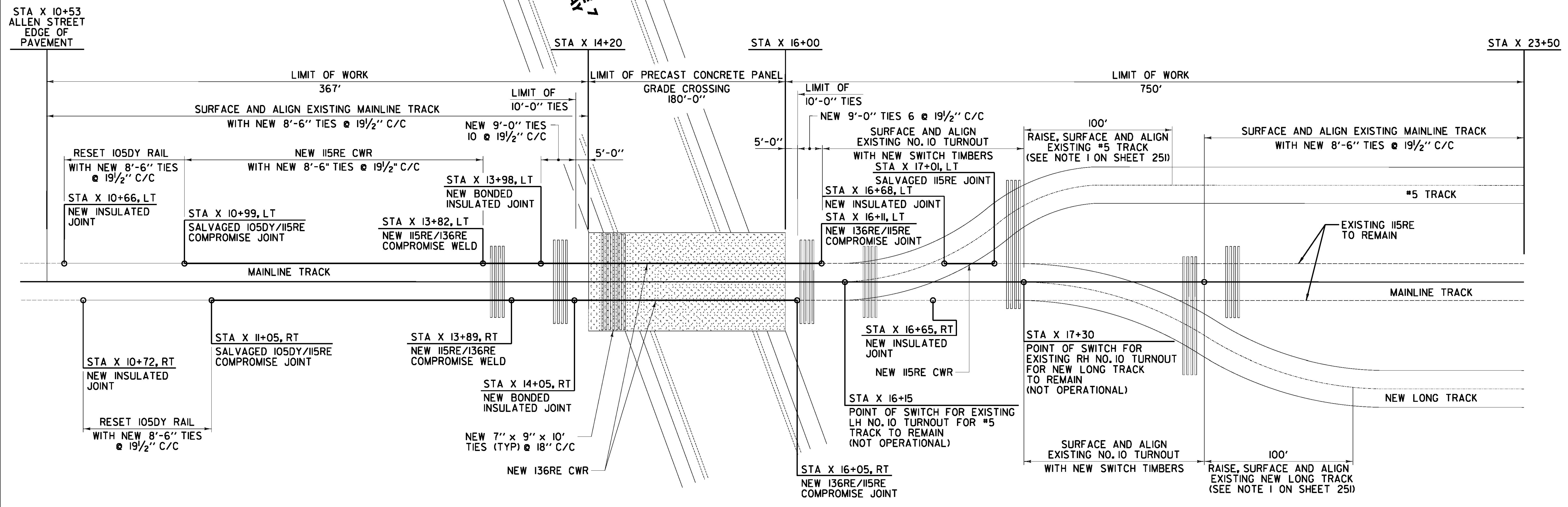
SCHEMATIC PLAN VIEW AARDOT 851-286U MP 0.48 HIGHWAY CROSSING
