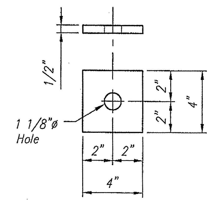
(P washer, 1/2" x 4" x 4") (Galvanized as per ASTM A153)
