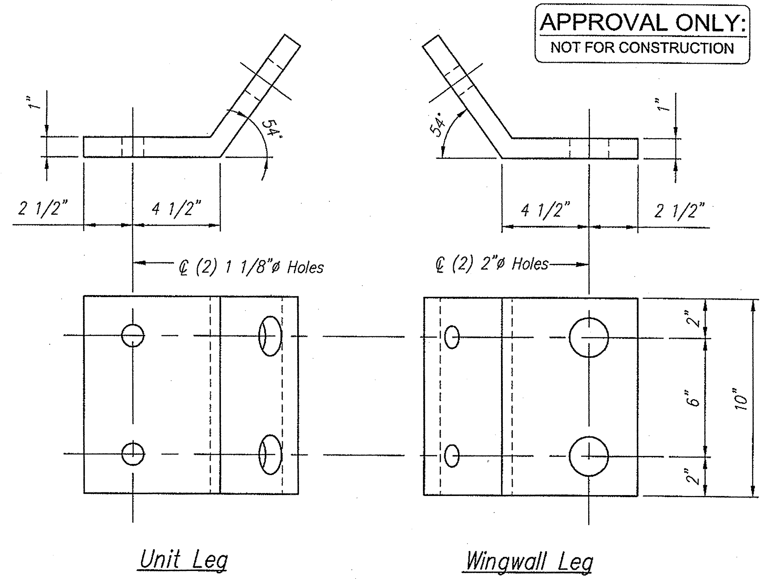
P-2 (P, 1" x 10" x 14") (Galvanized as per ASTM A153)
