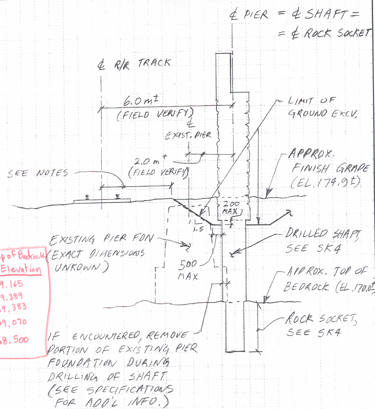
PIER TYPICAL SECTION SCALE = 1"=100'
