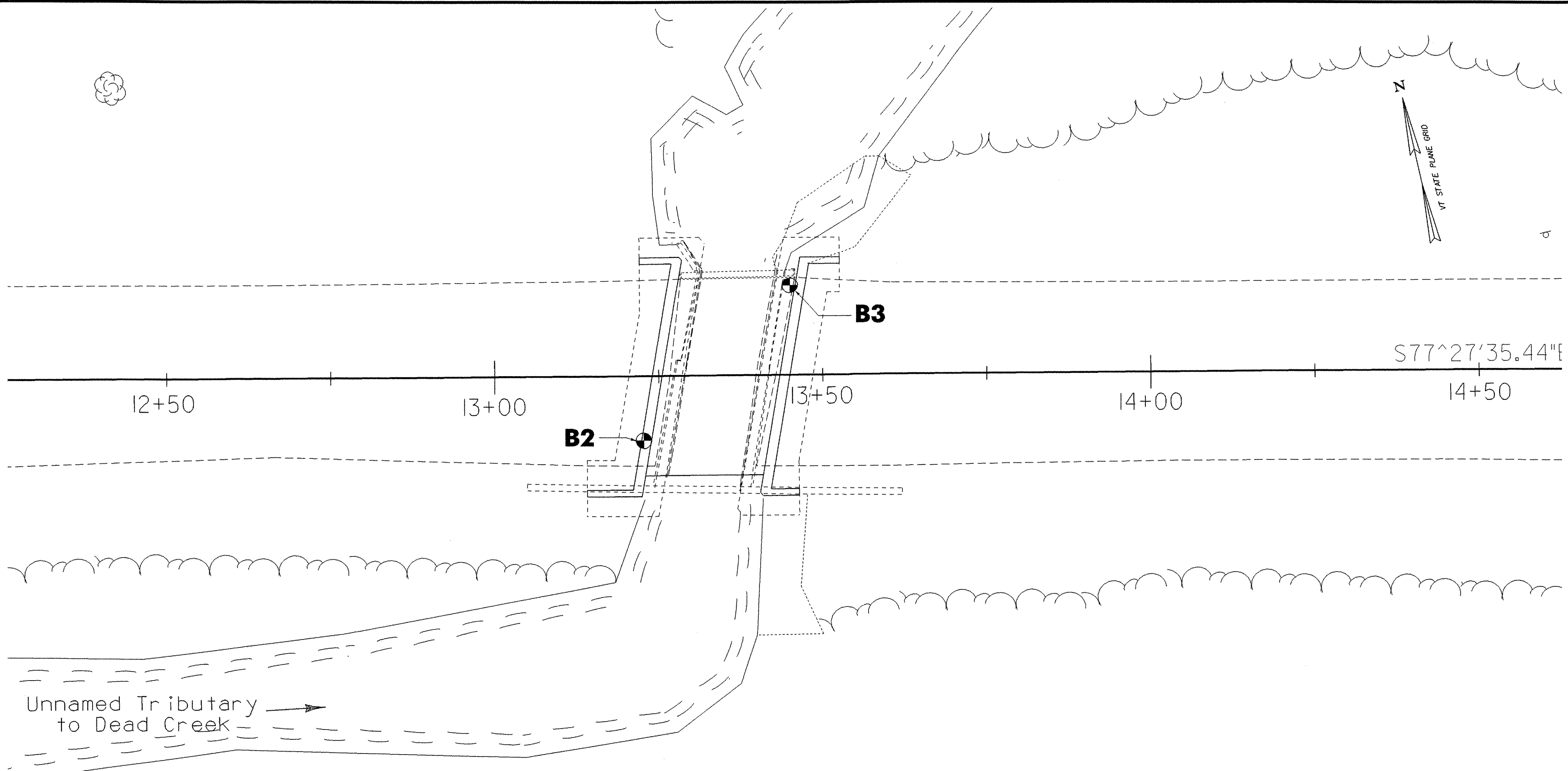
BORING CHART
