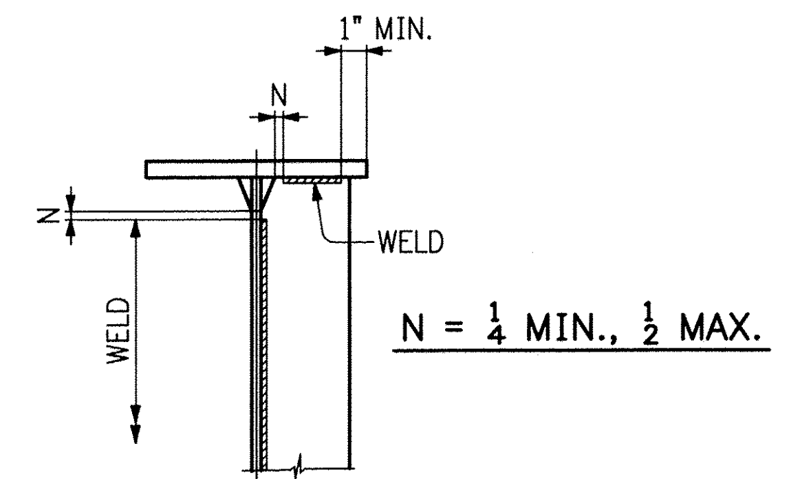
TYP. WELD TERMINATION DETAIL
