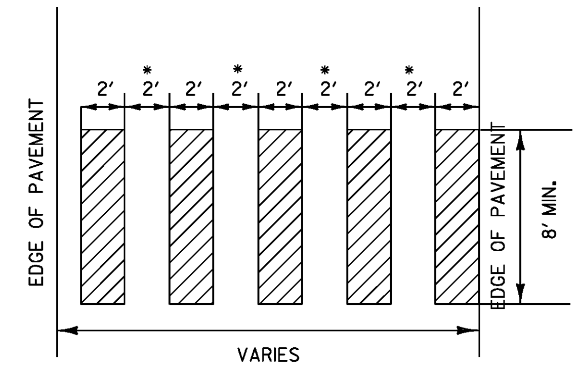
BLOCK PATTERN CROSSWALK DETAIL
