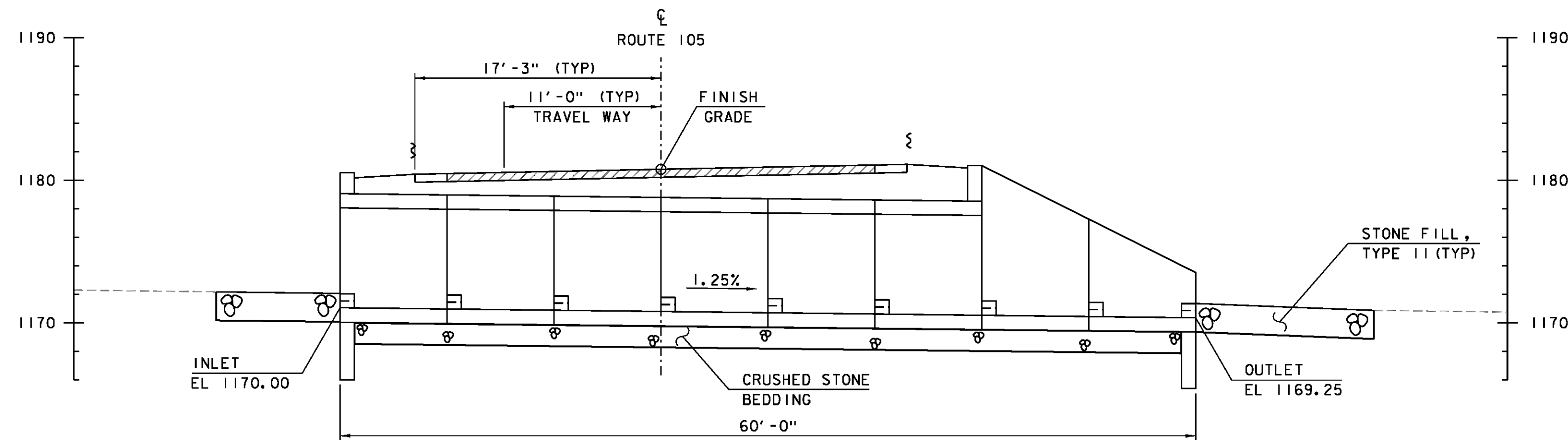
CHANNEL PROFILE ALONG \xi BOX SCALE 1" = 5'-0"
