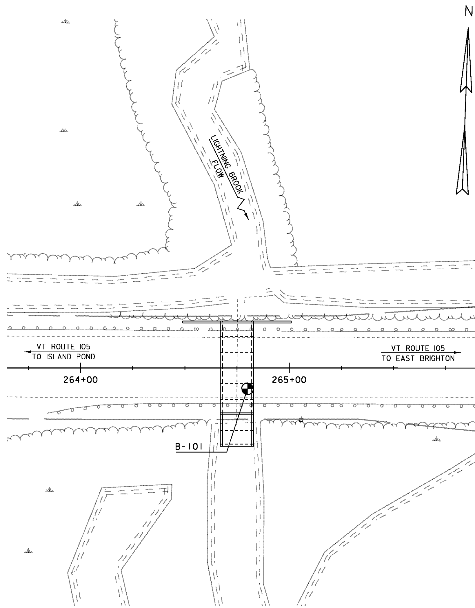
BORING LAYOUT SCALE 1" = 20' - 0" 20 0 20
