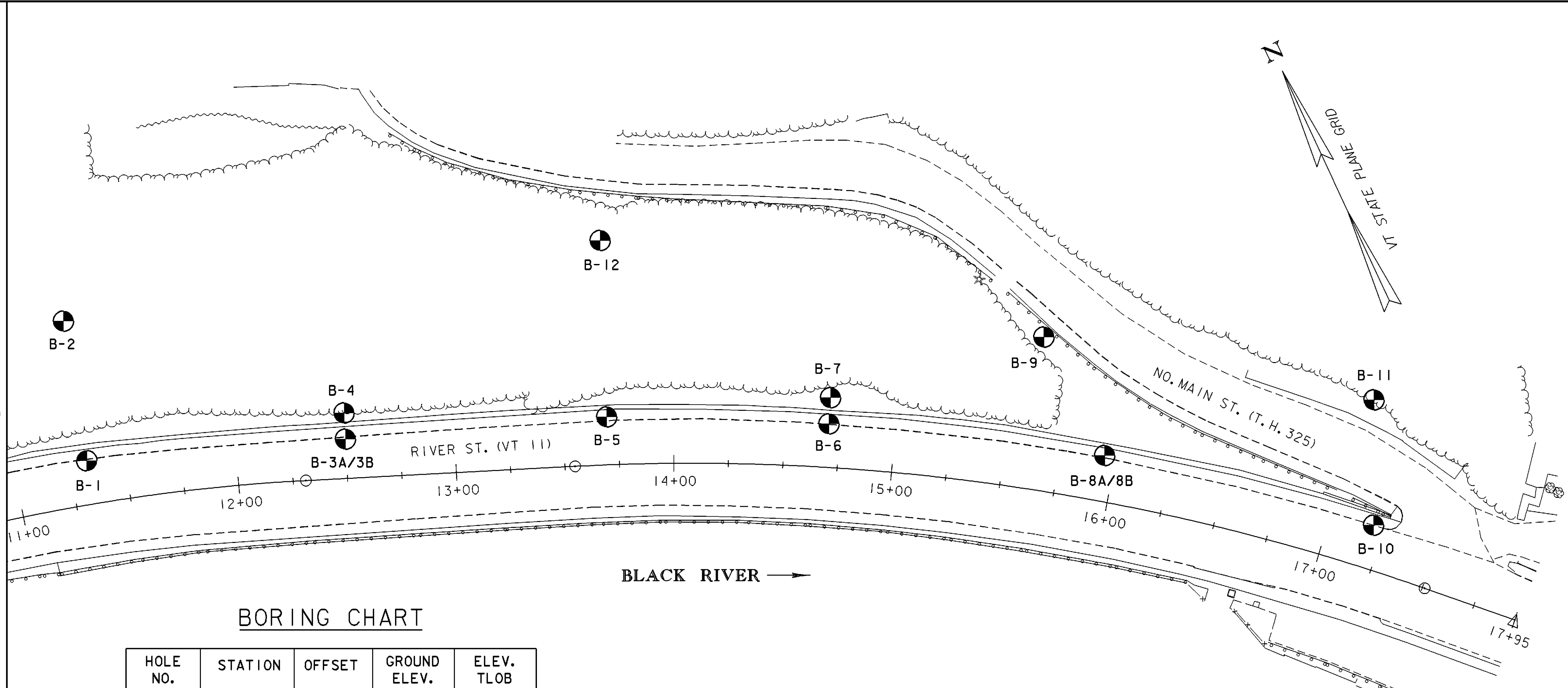
BORING PLAN
