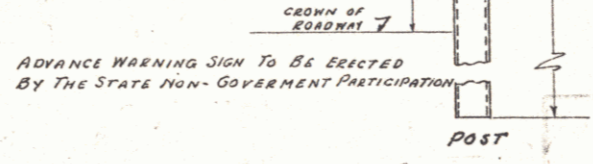
RAILROAD ADVANCE WARNING SIGN SCALE 1"=10'
