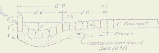
GRAUTED COBBLE GUTTER 170+50-171+40 STA 101+30-101+75
