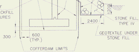
TYPICAL NEW ABUTMENT SECTION NOT TO SCALE
