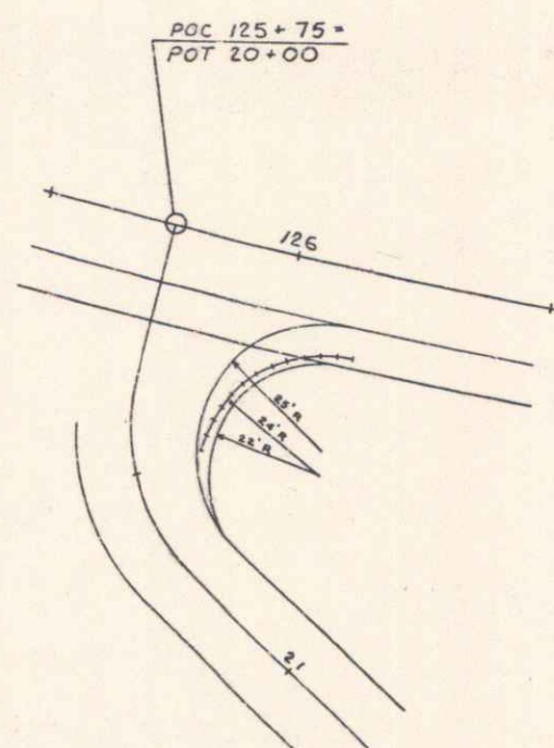
Detail of Guard Rail (3' 1/2" Spacing) 125+31.1 - 126+14.3 RT See Sheet 9 of 73 Scale 1" = 20 feet
