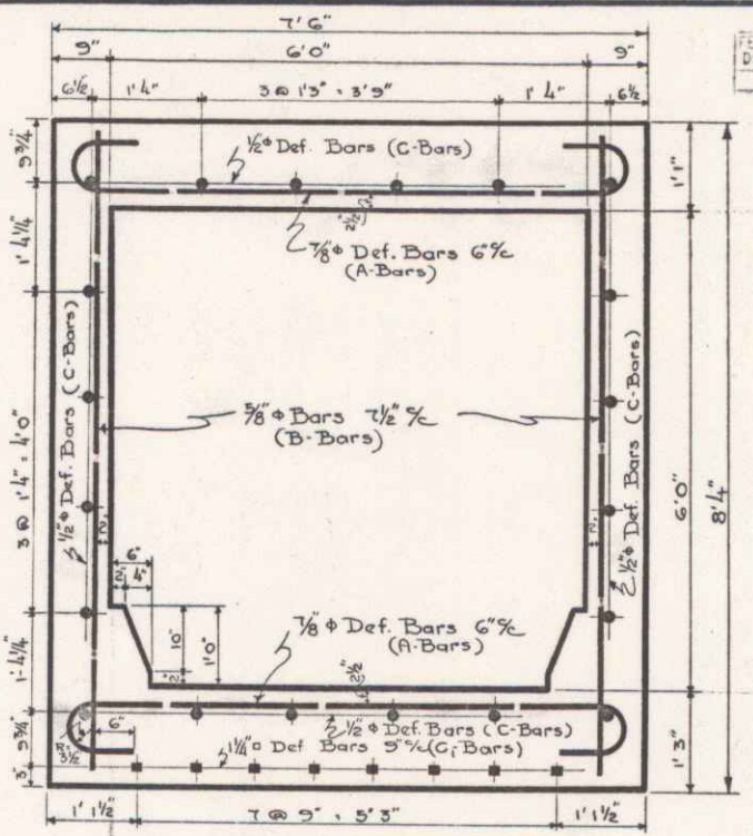
CROSS SECTION of 6x6 R.C. Box STA. 32+36 Showing detail of concrete and steel in Barrel. For details of wings see Standard sheet 5C1.
