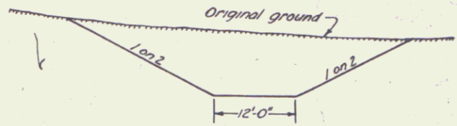
Sketch showing proposed channel relocation Lt. of sta 562+50 to sta 574+00
