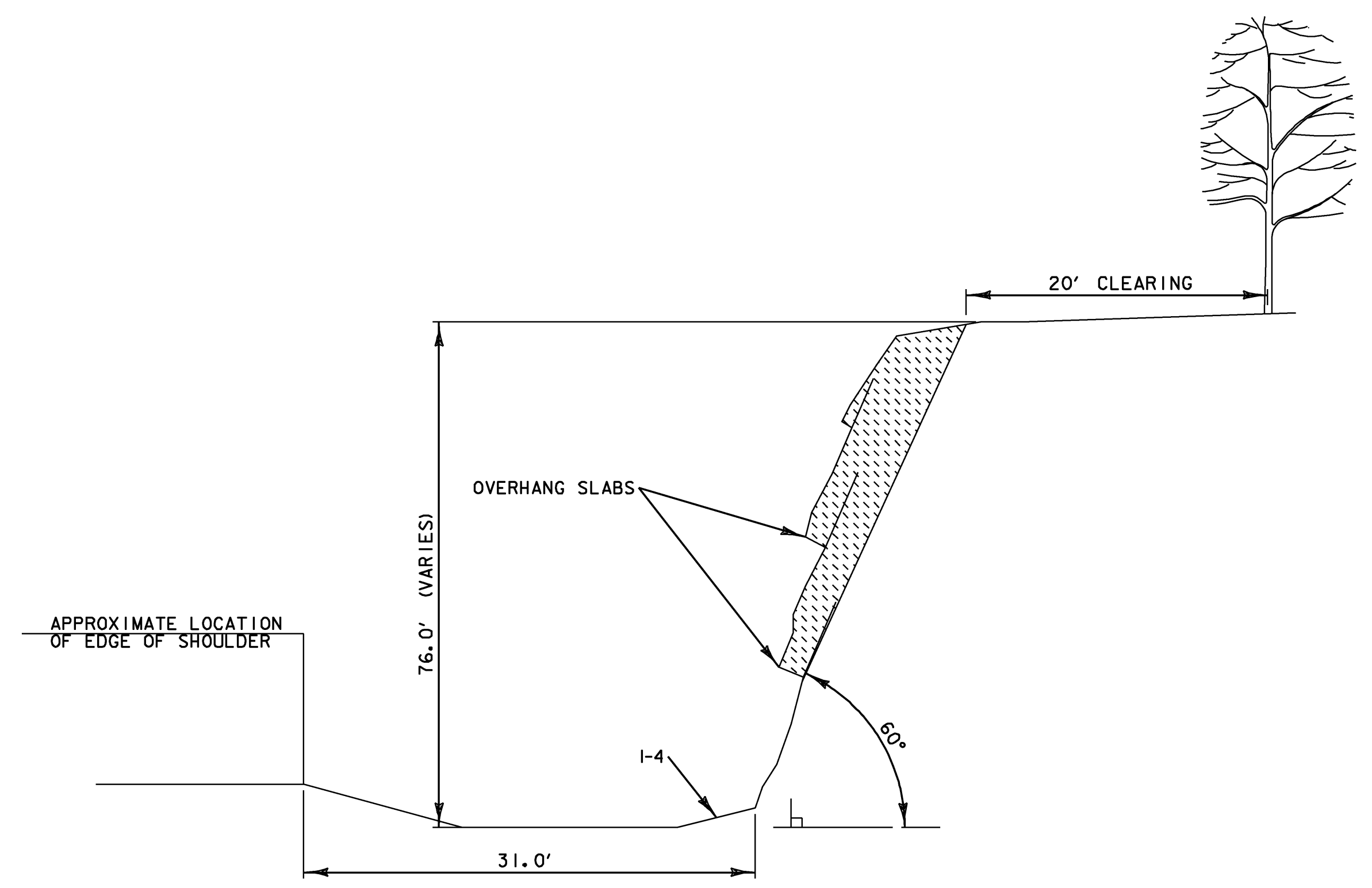
A 14 SCHEMATIC - CROSS SECTION
