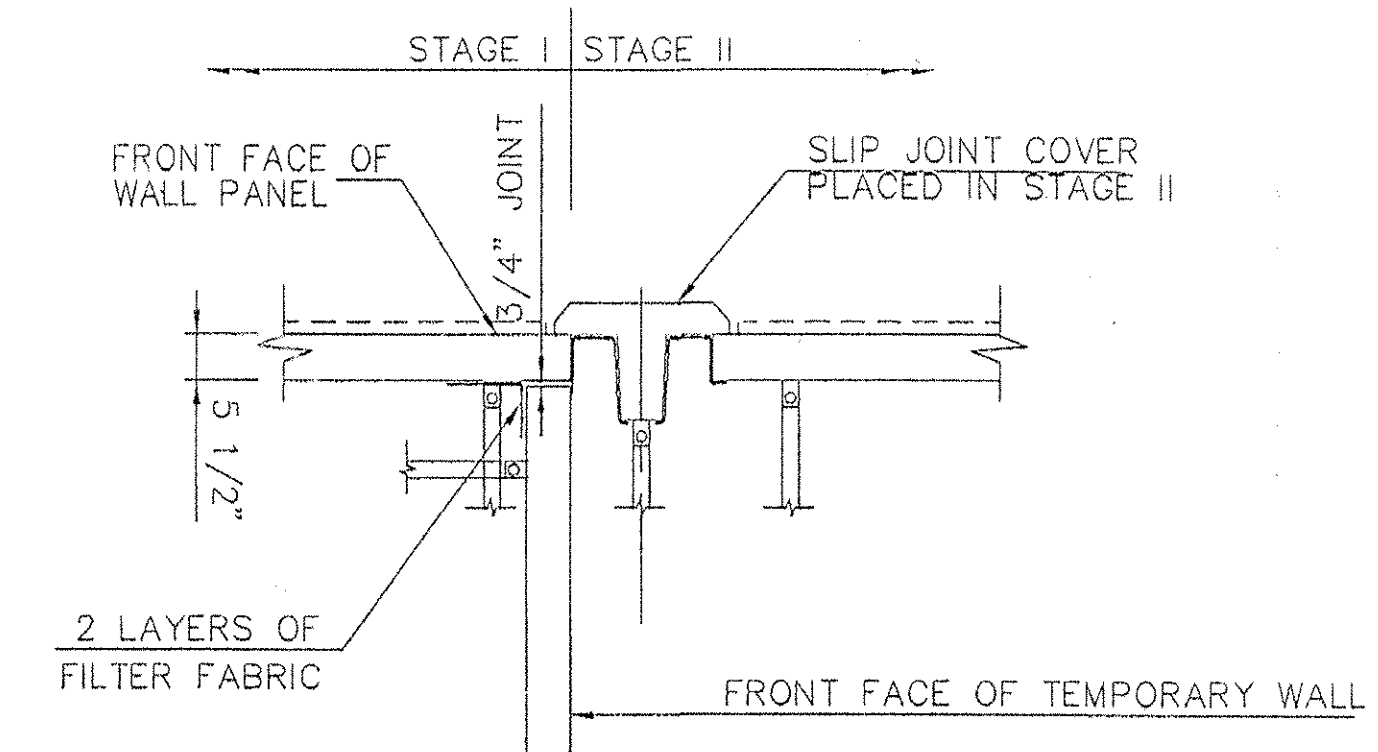
STAGED CONSTRUCTION DETAIL SCALE: 1/2" = 1'-0"
