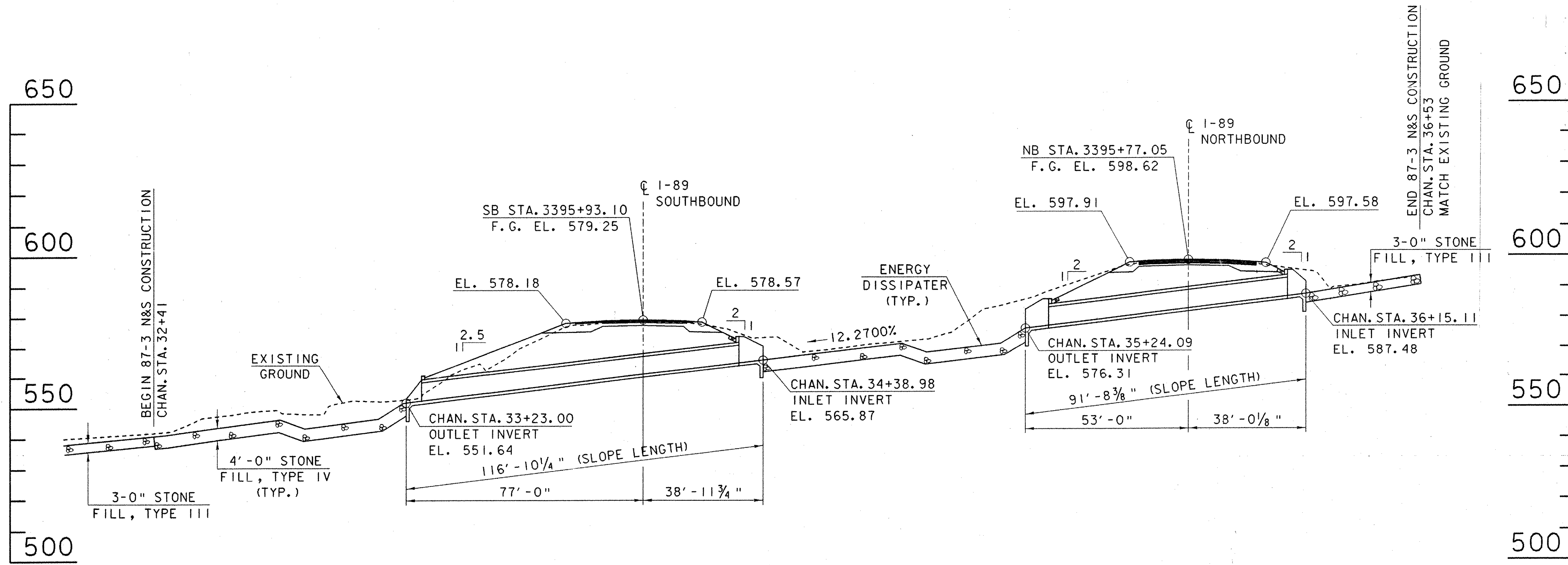
BRIDGES 87-3 N&S ELEVATION ALONG \phi CULVERTS
