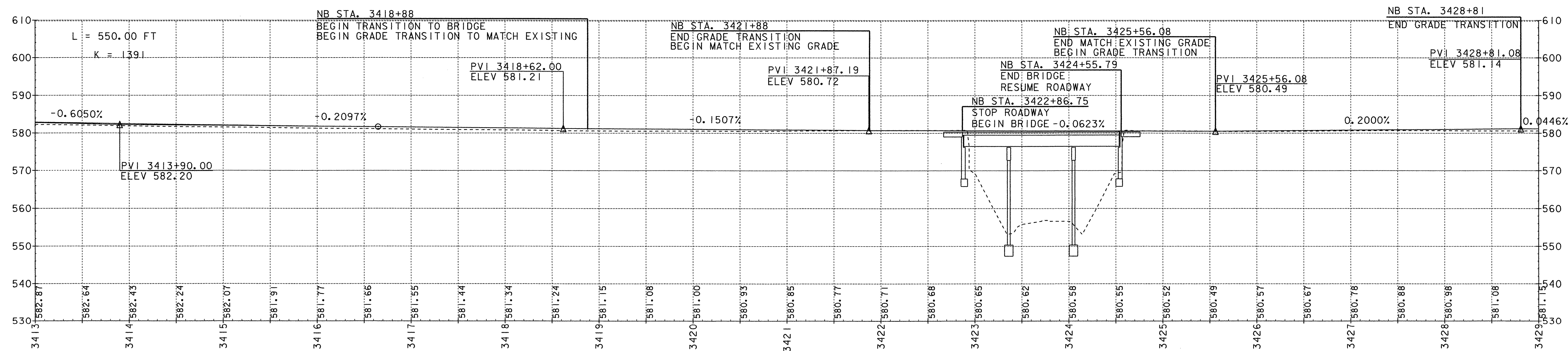
NORTHBOUND GRADE PROFILE ALONG MEDIAN SIDE (REFER TO TYPICAL SHEET) STA. 3413+00 - 3429+00
