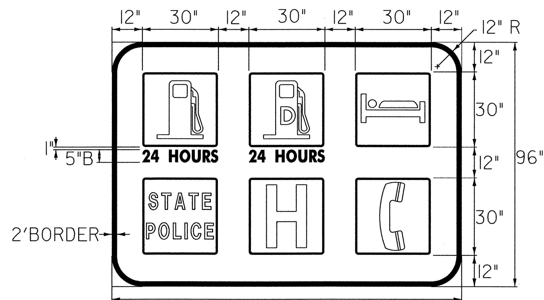
VD 367 WHITE SYMBOLS, BORDER & TEXT WITH BLUE BACKGROUND MM 113.21 NB.
