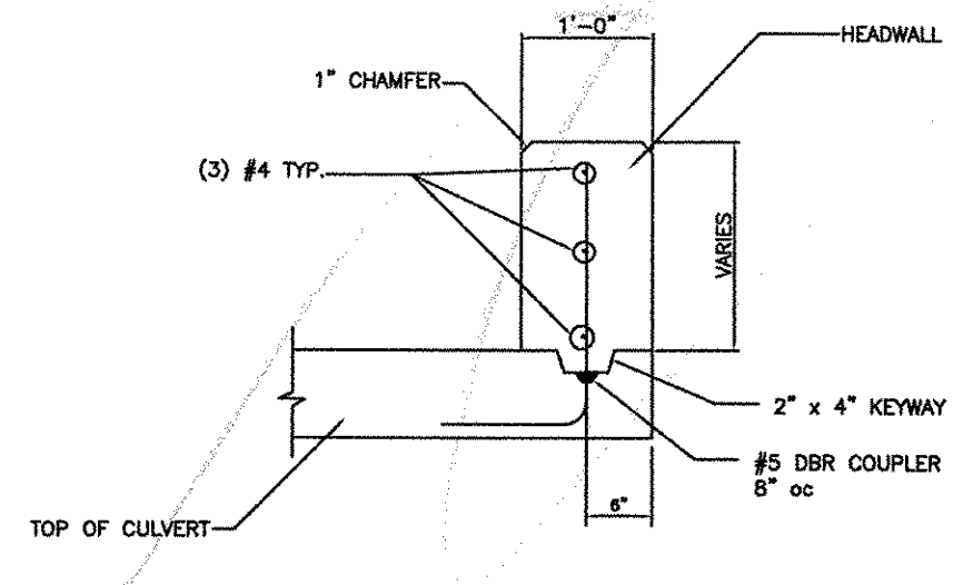
HEADWALL DETAIL
