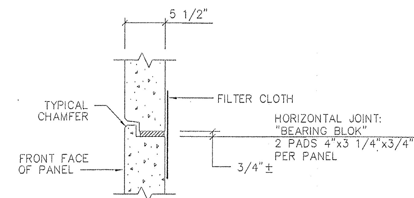
SECTION 1-1
