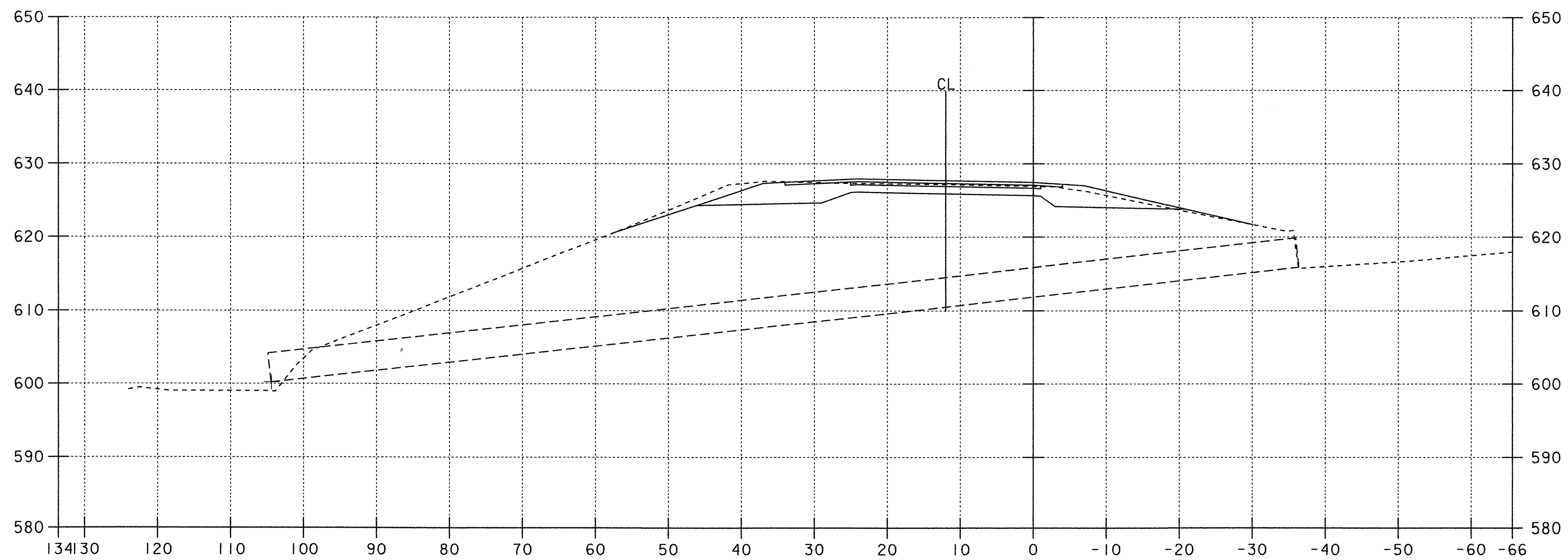
3334+18 EXISTING 48' ACCGMP
