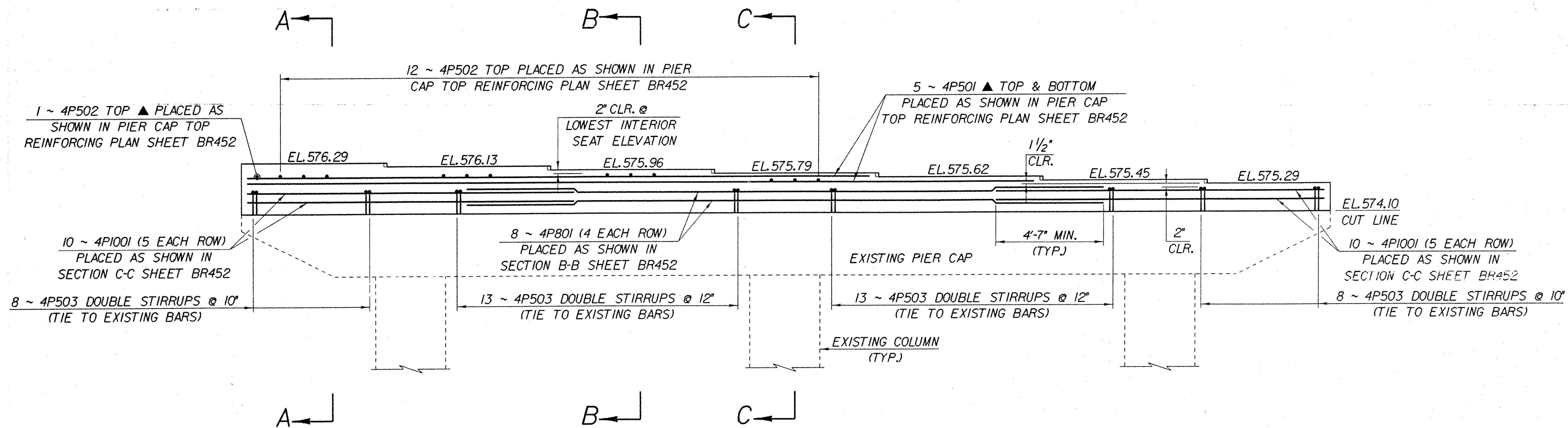
PIER NO. 4 PARTIAL ELEVATION
