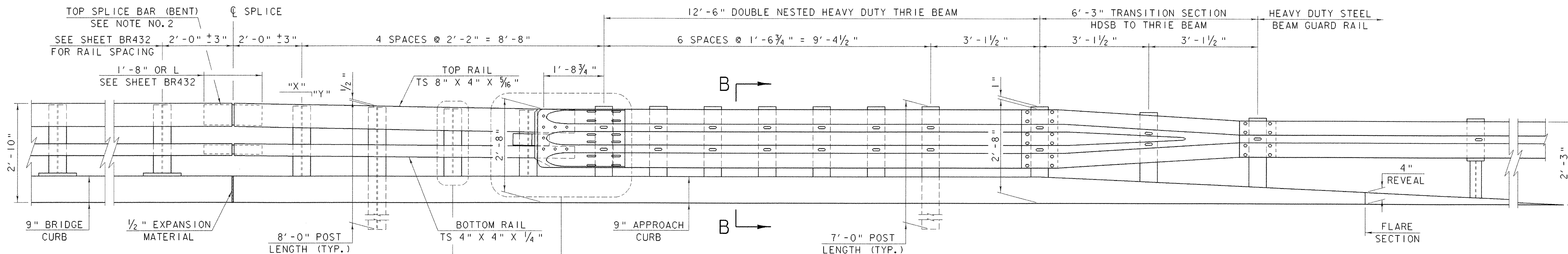
APPROACH RAIL SLOPE
