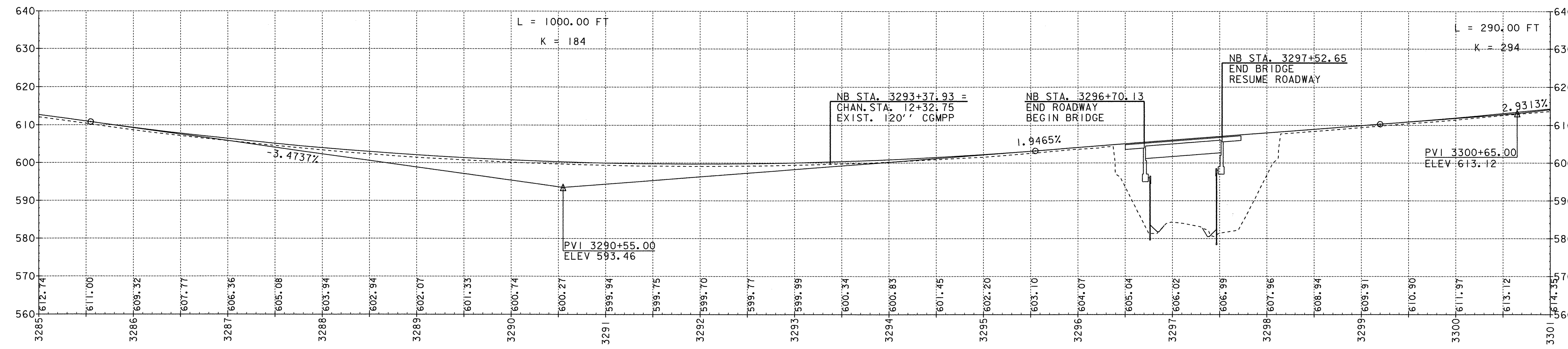
NORTHBOUND GRADE PROFILE ALONG MEDIAN SIDE (REFER TO TYPICAL SHEET) STA. 3285+00 - 3301+00
