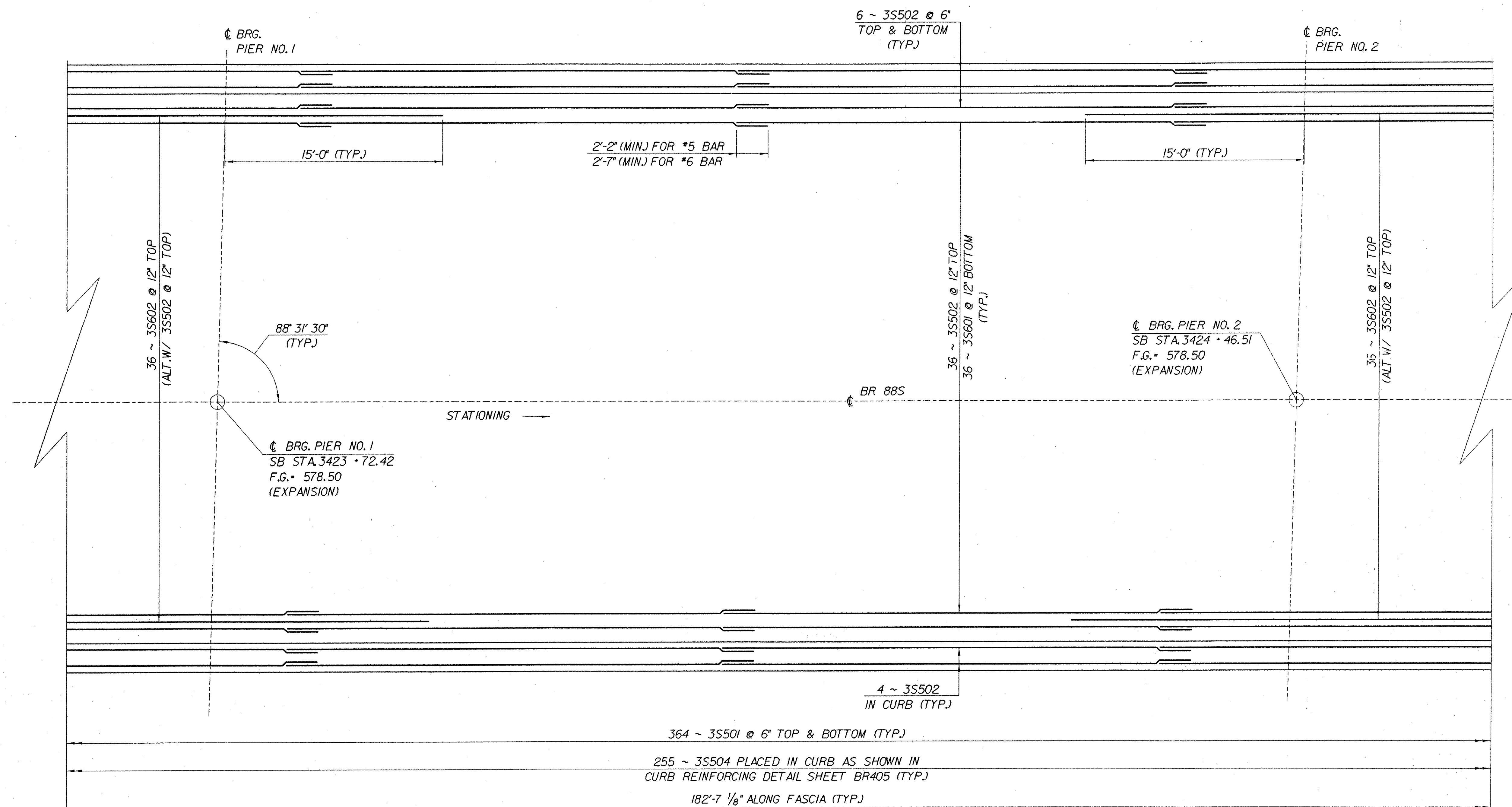
BRIDGE 88S DECK REINFORCING PLAN SPAN TWO SCALE: 1/4" = 1' - 0"
