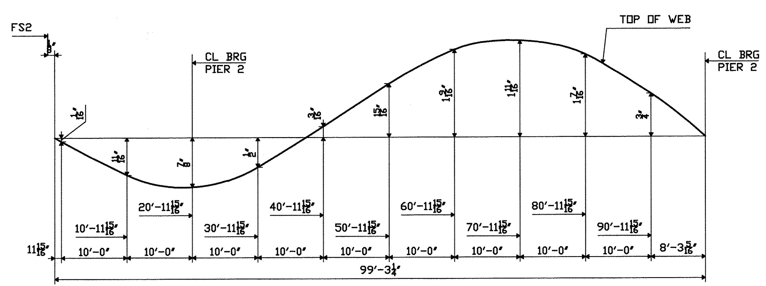
CAMBER DIAGRAM
