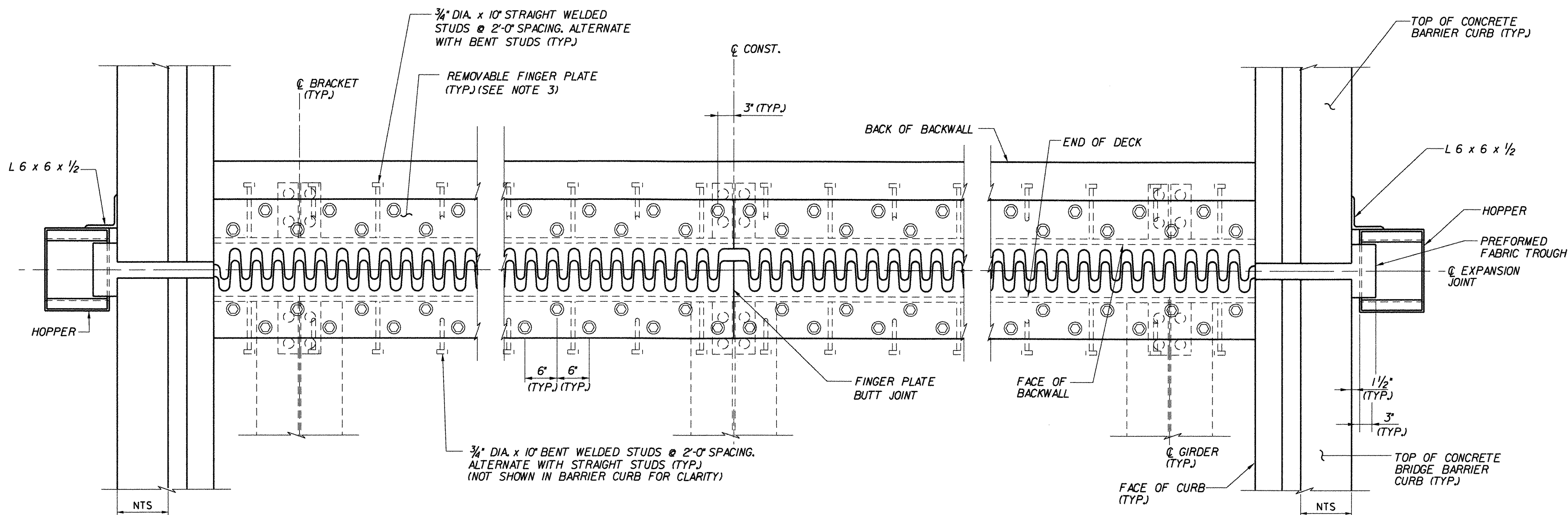
FINGER PLATE EXPANSION JOINT PLAN (3S)
