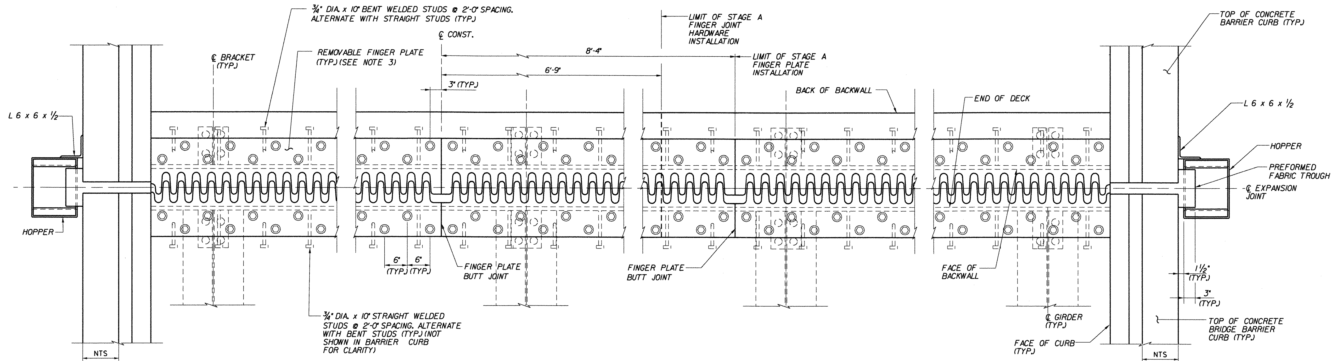
FINGER PLATE EXPANSION JOINT PLAN (3N)
