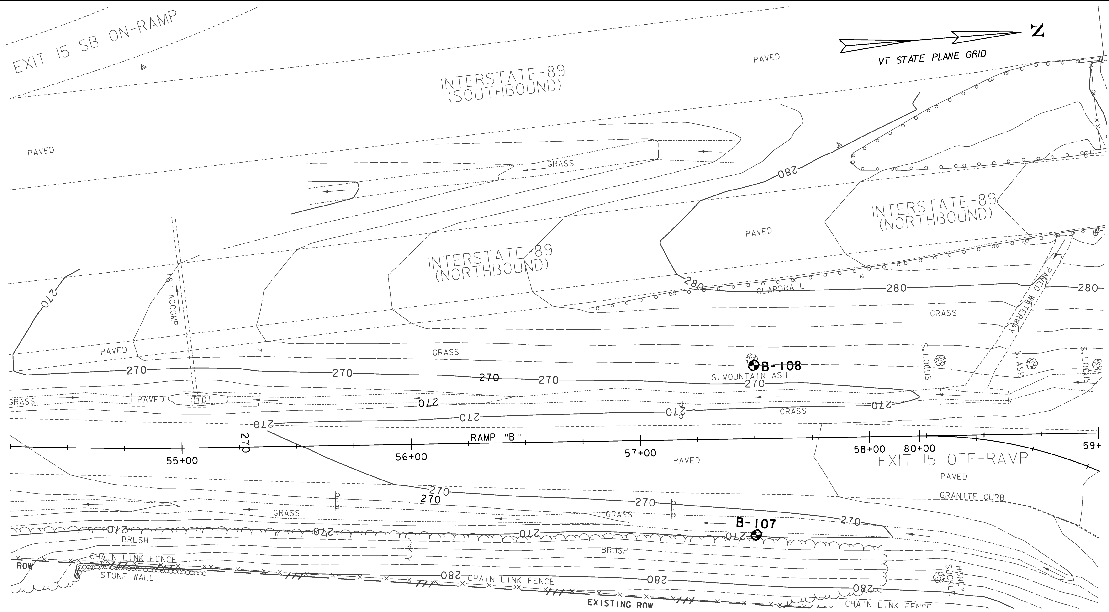
BORING LAYOUT
