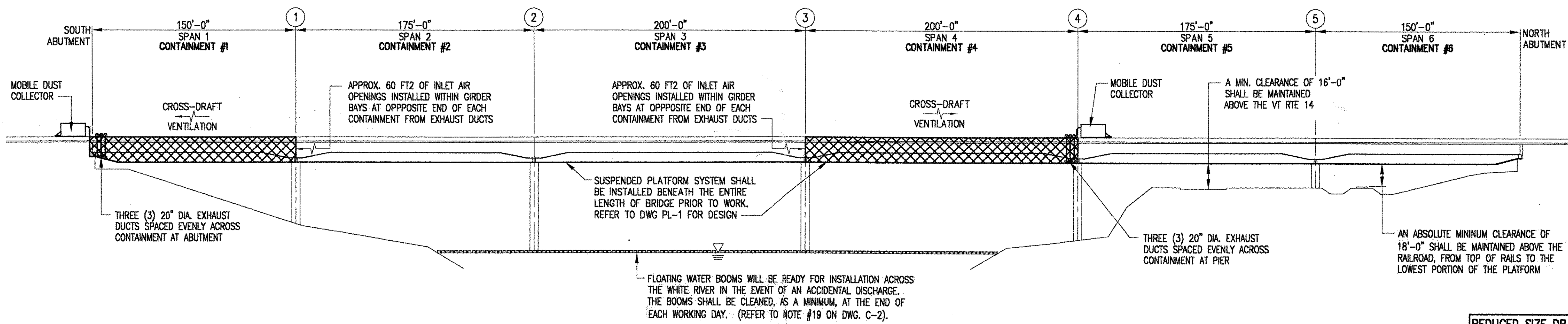
ELEVATION NORTHBOUND AS SHOWN - SOUTHBOUND IDENTICAL SCALE: 1" = 40'-0"
