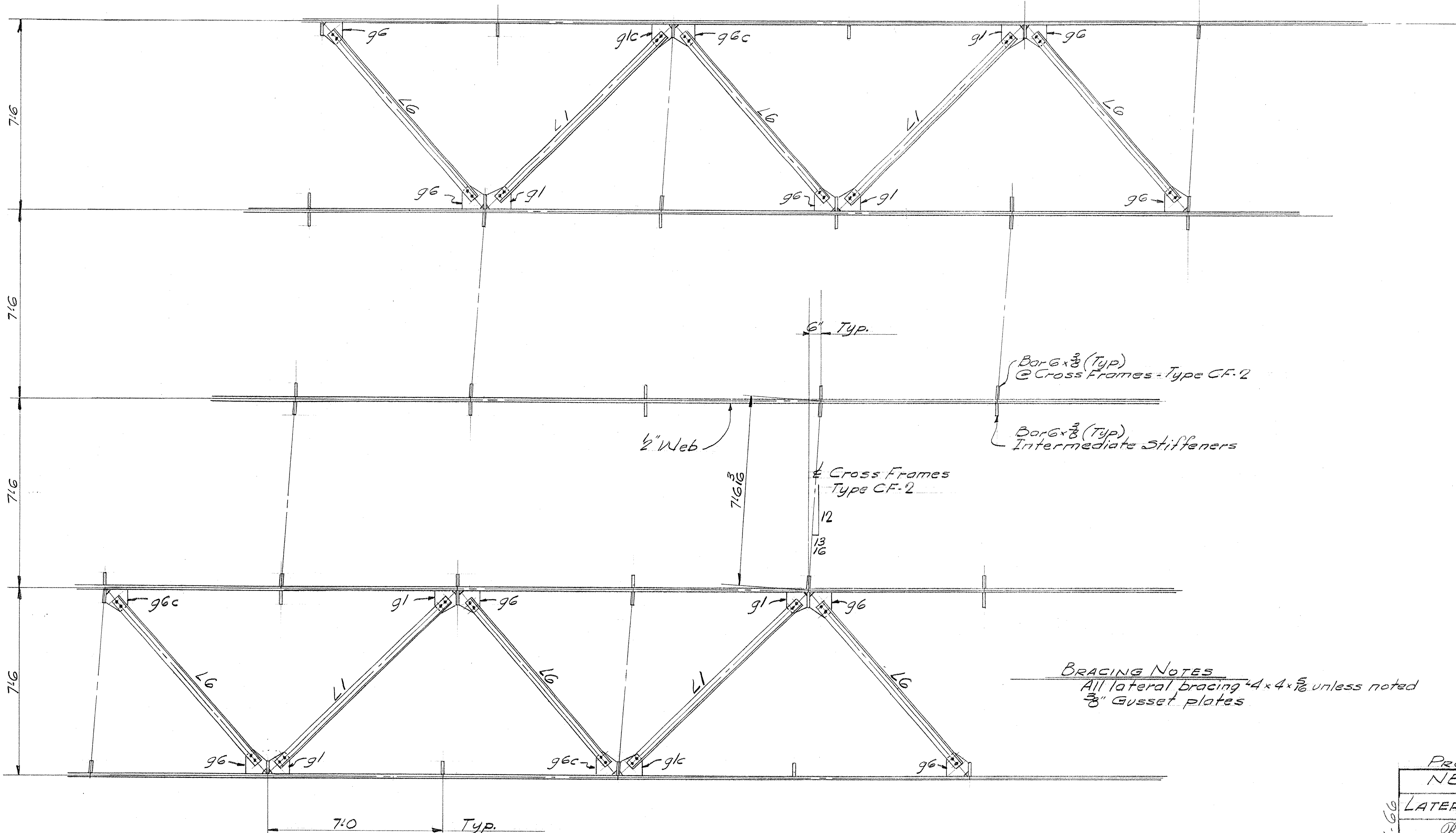
PLAN OF LATERAL BRACING @ SPANS 2-3-4 & 5 Cross Frames not shown.
