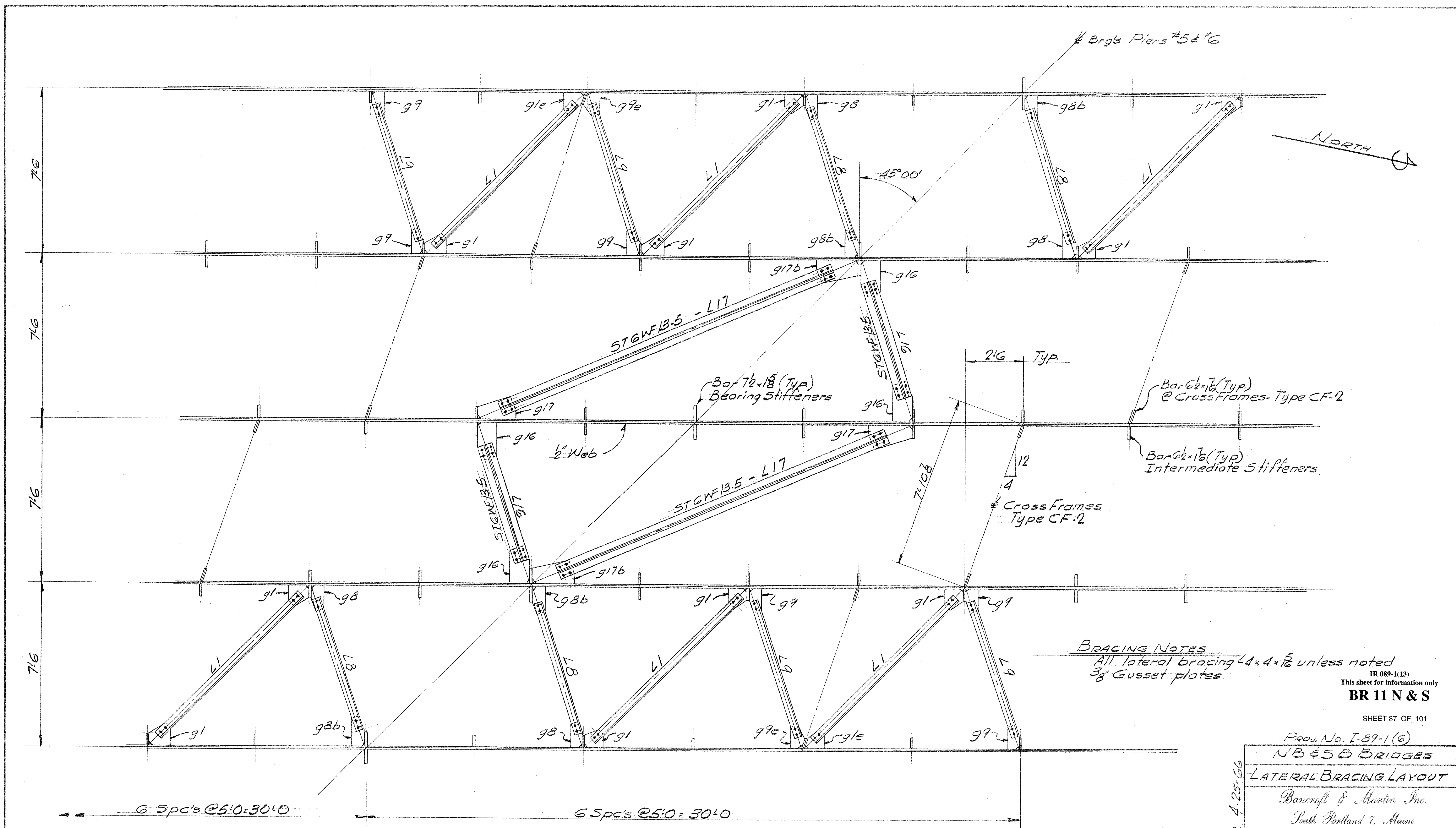
PLAN OF LATERAL BRACING @ PIERS #5 & #6 Cross Frames & Longitudinal Stiffeners not shown.
