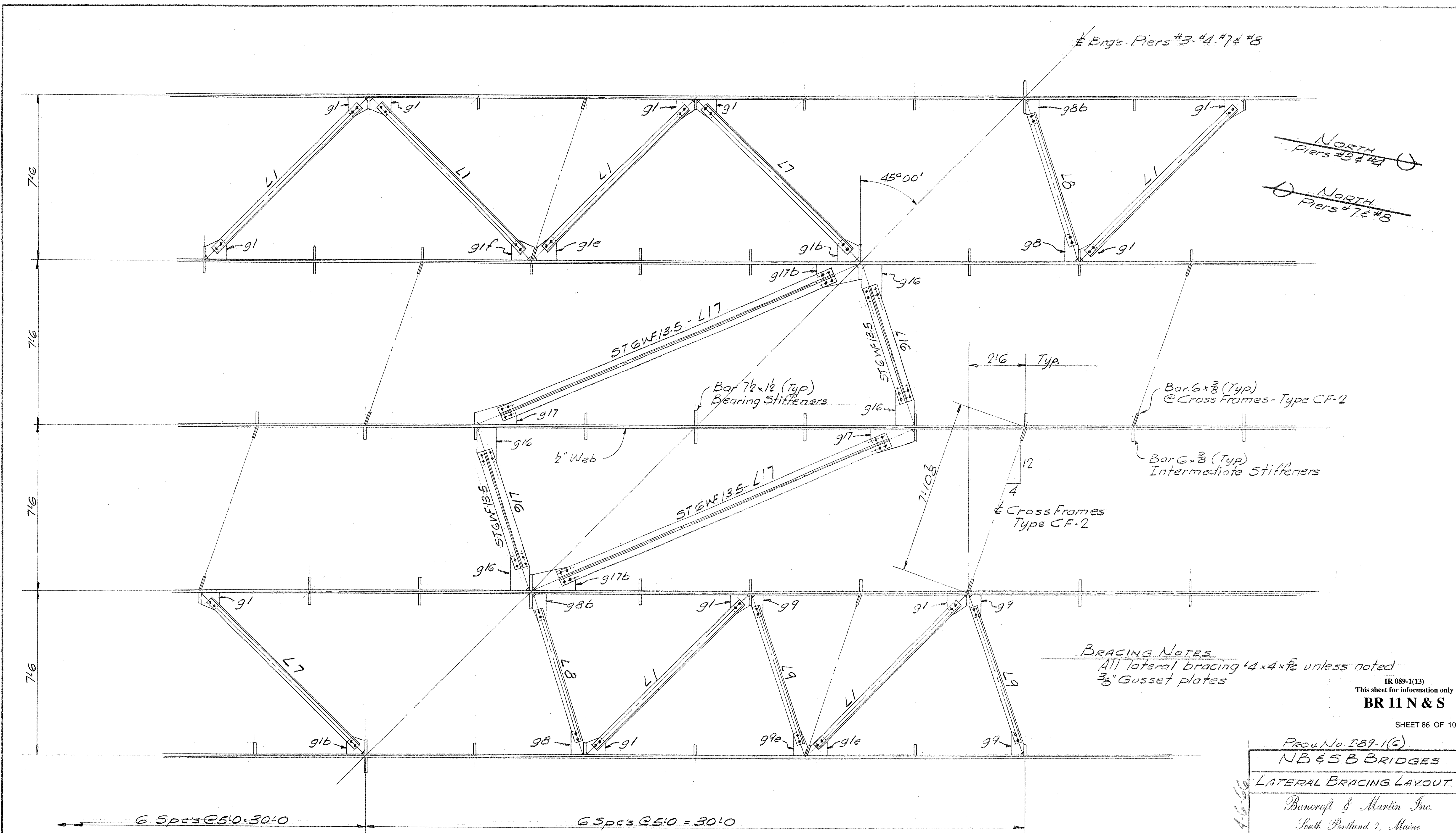
PLAN OF LATERAL BRACING @ PIERS #3-#4-#7-#8 Cross Frames & Longitudinal Stiffeners not shown.
