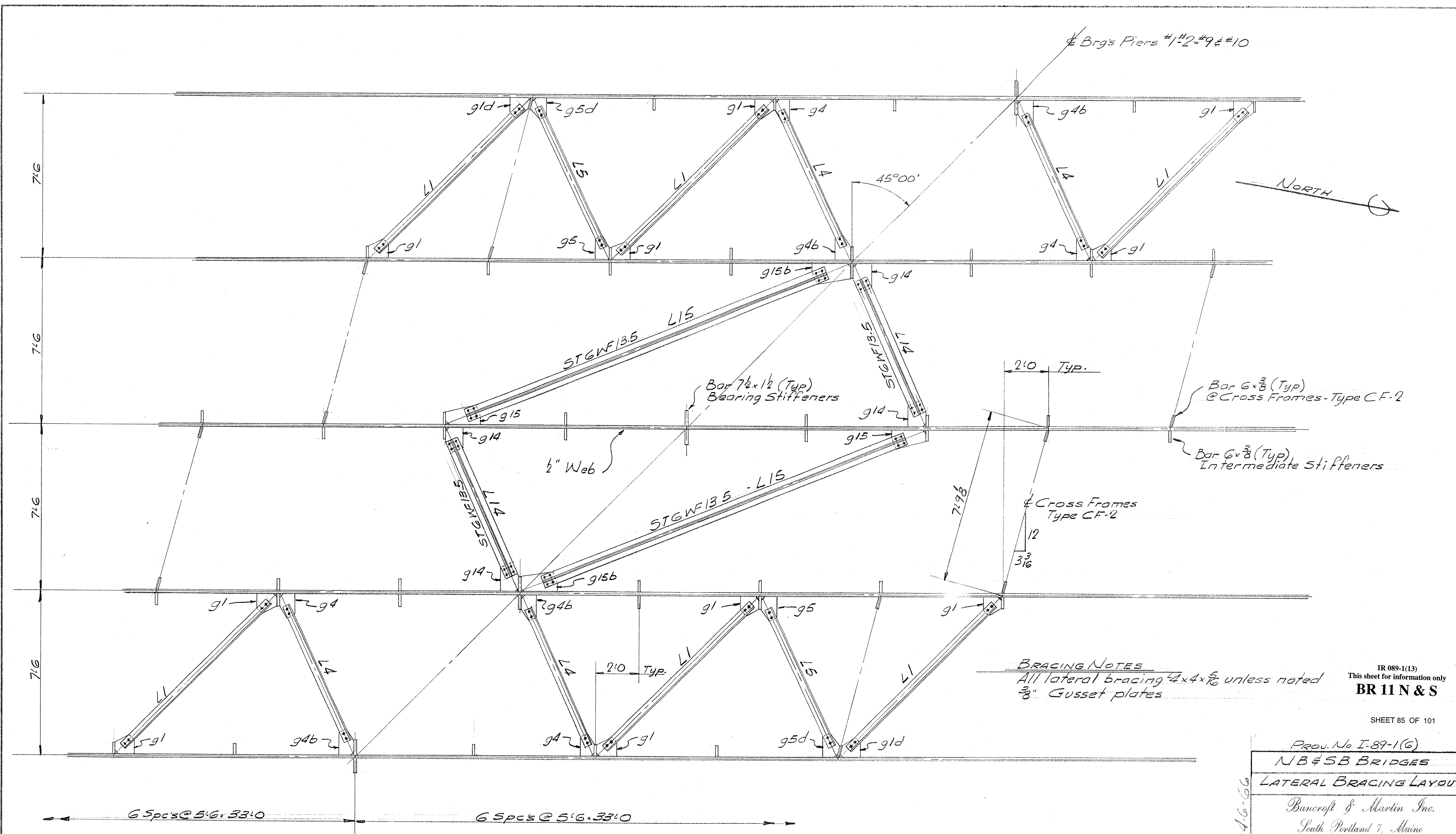
PLAN OF LATERAL BRACING @ PIERS #1-#2-#9 & #10 Cross Frames & Longitudinal Stiffeners not shown.
