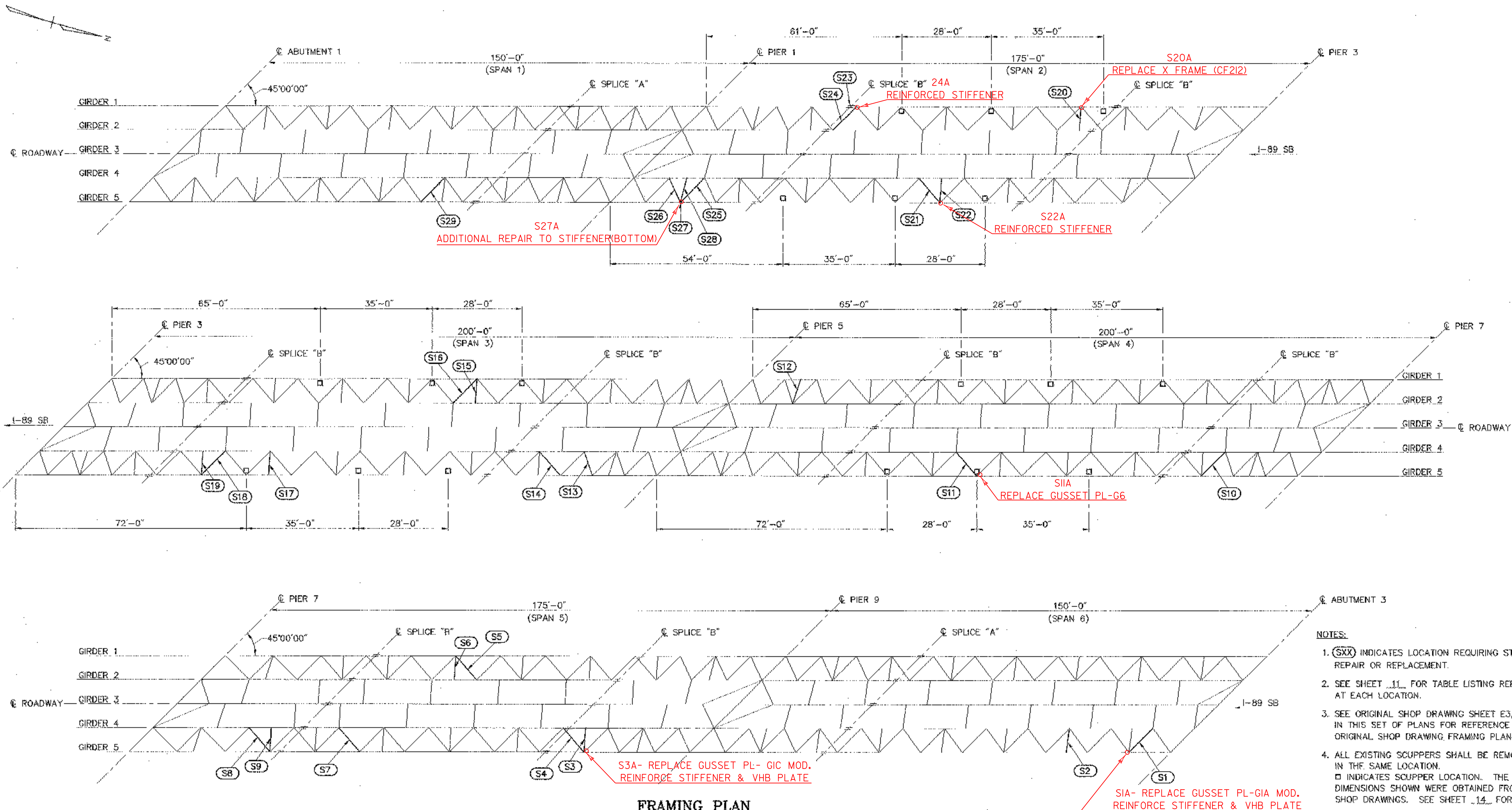
FRAMING PLAN SCALE: 1/16" = 1'-0"
