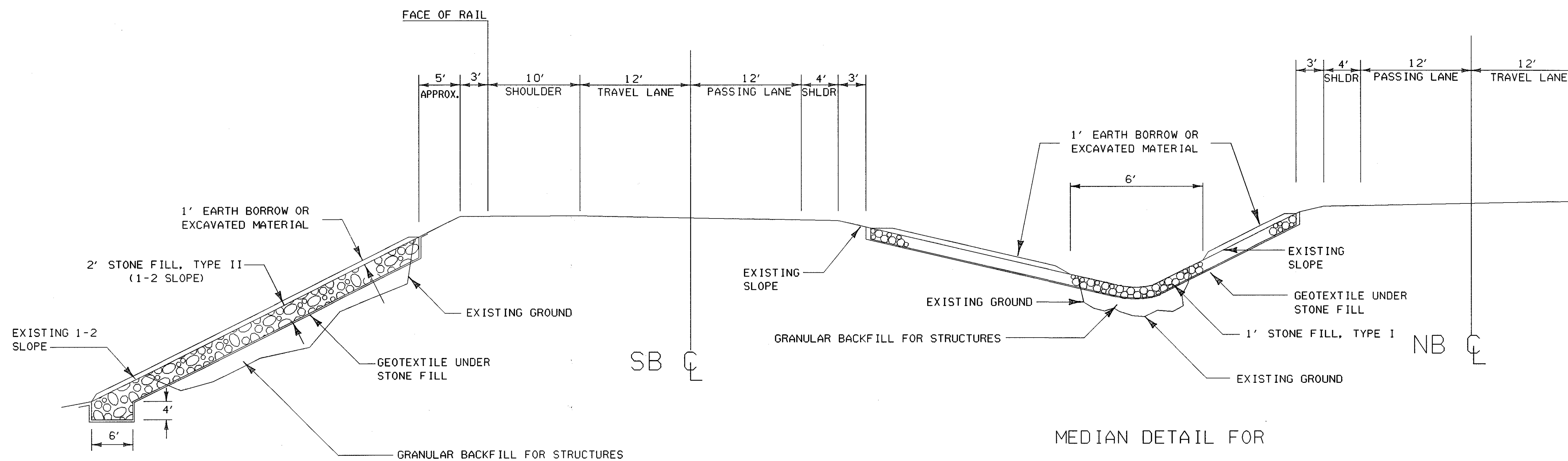
SIDE SLOPE DETAIL FOR MM 7.28 - 7.31 & MM 7.34 - 7.39
