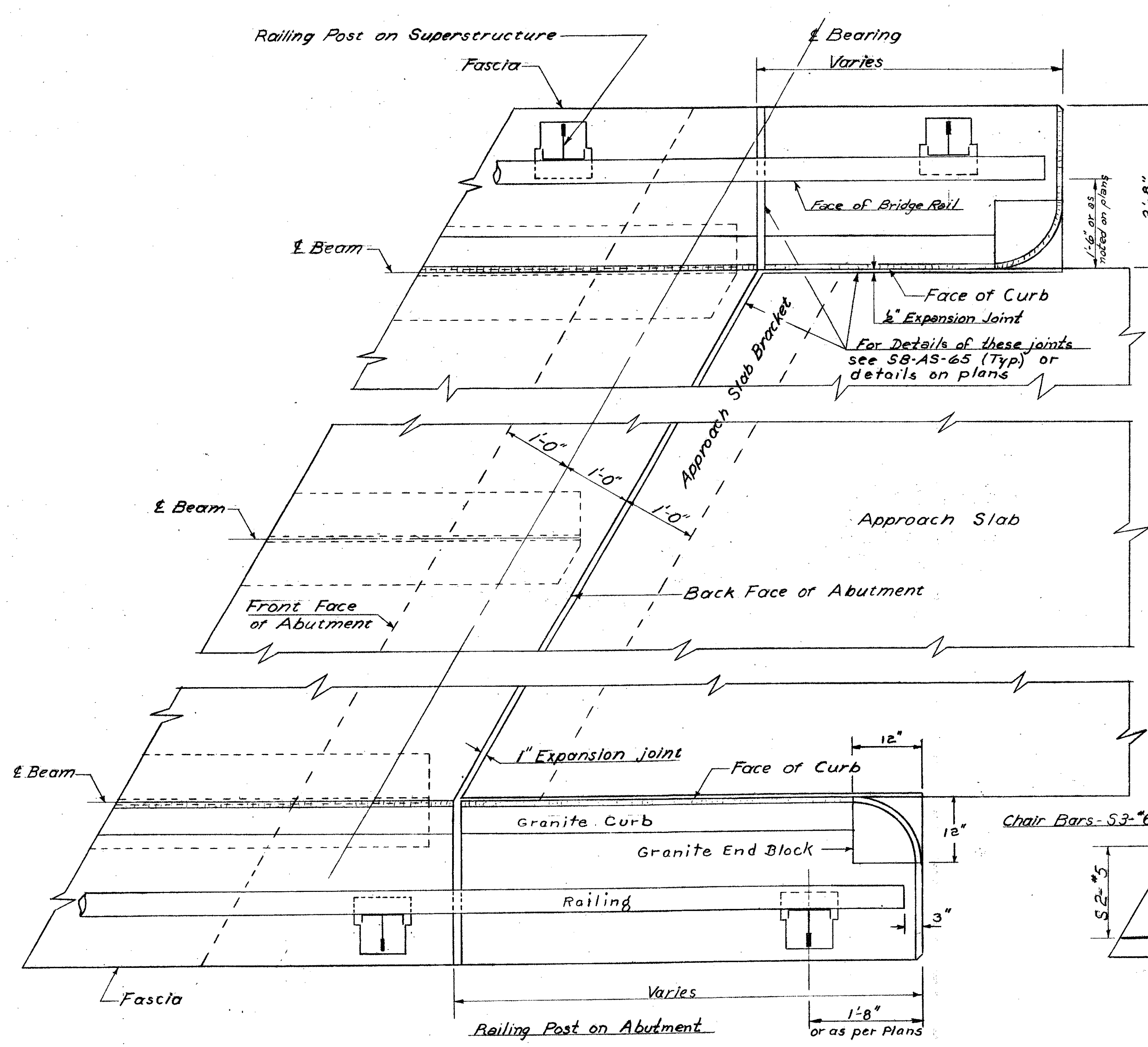
PLAN AT ABUTMENT
