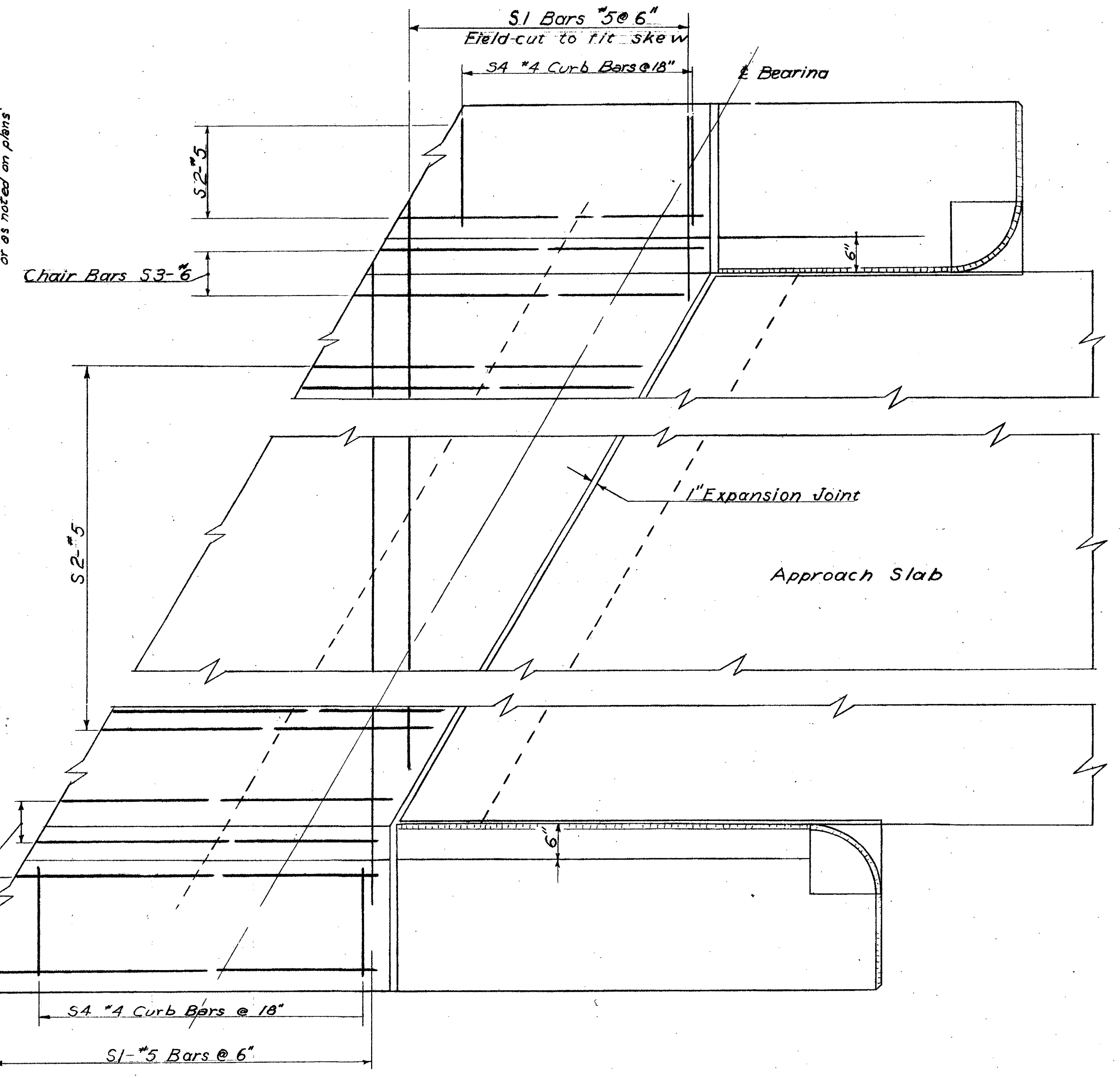
REINFORCEMENT LAYOUT AT ABUTMENT
