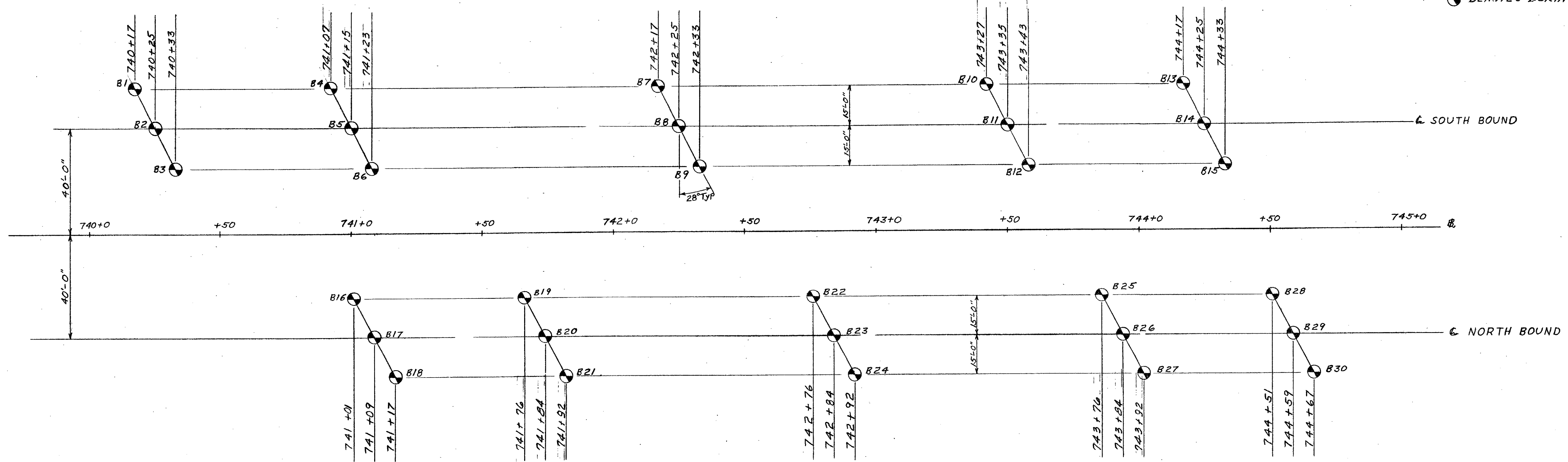
BORING PLAN SCALE 1" = 20'
