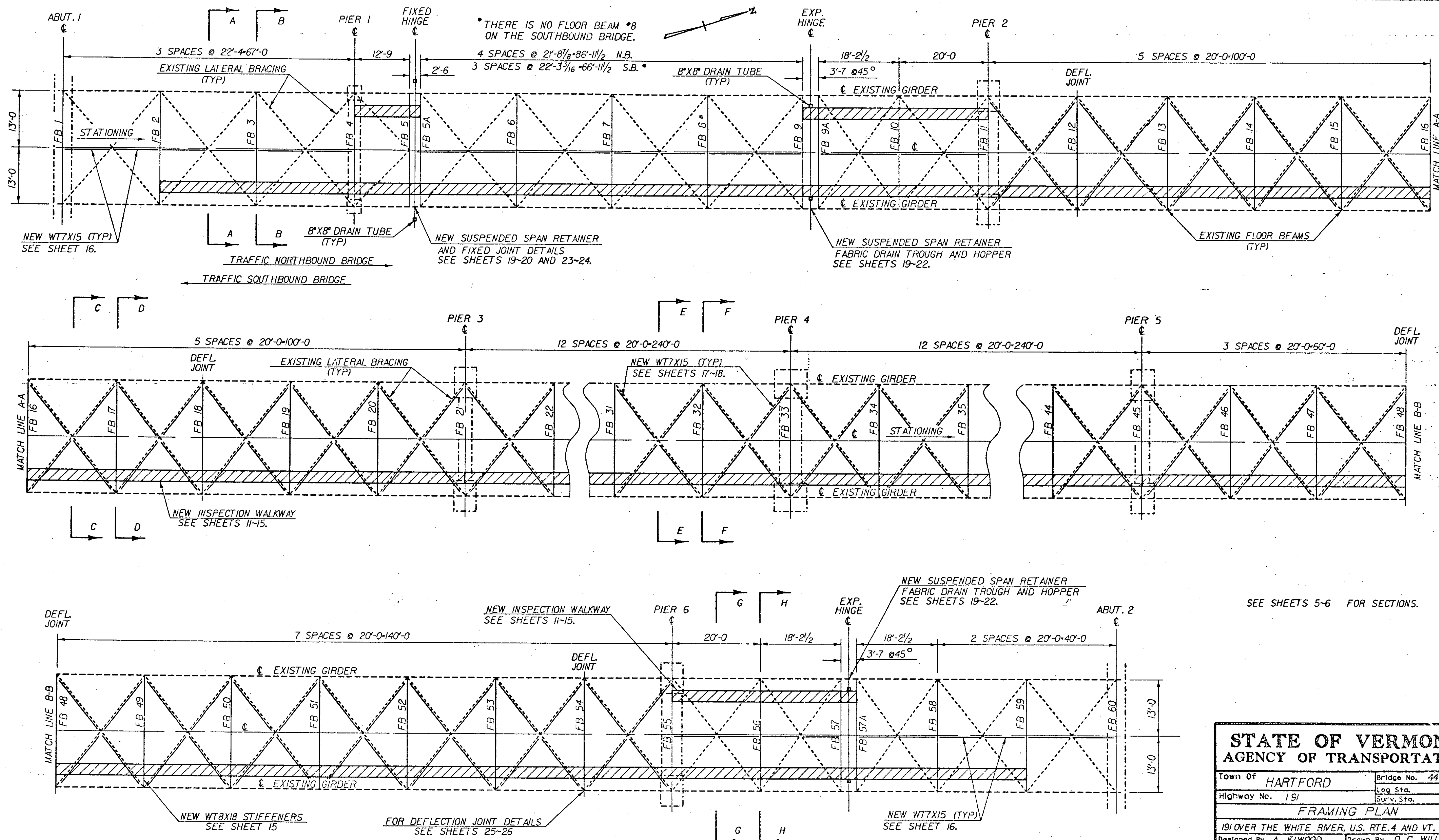
FRAMING PLAN SCALE 1"=10'
