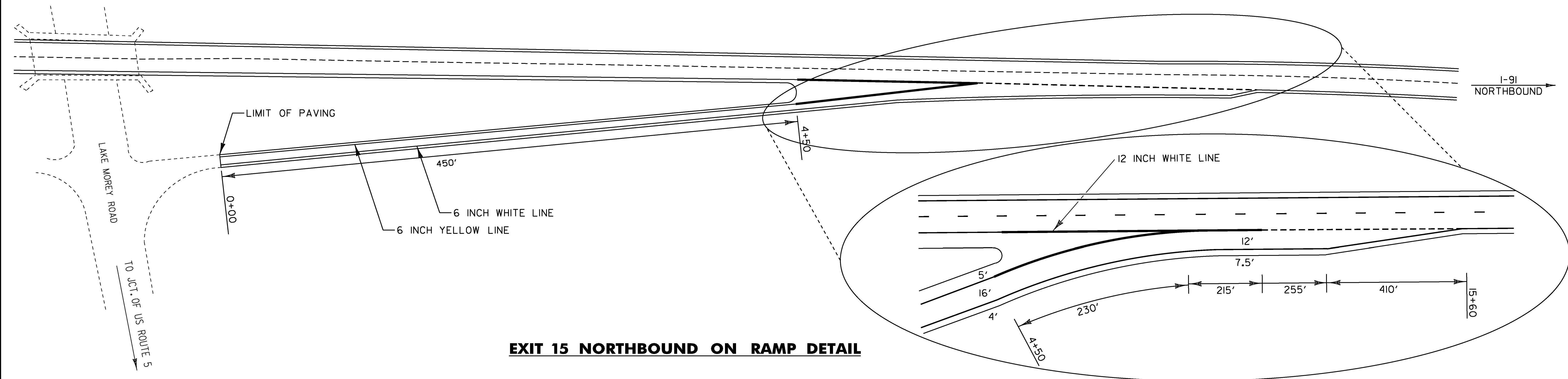
EXIT 15 NORTHBOUND OFF RAMP DETAIL
