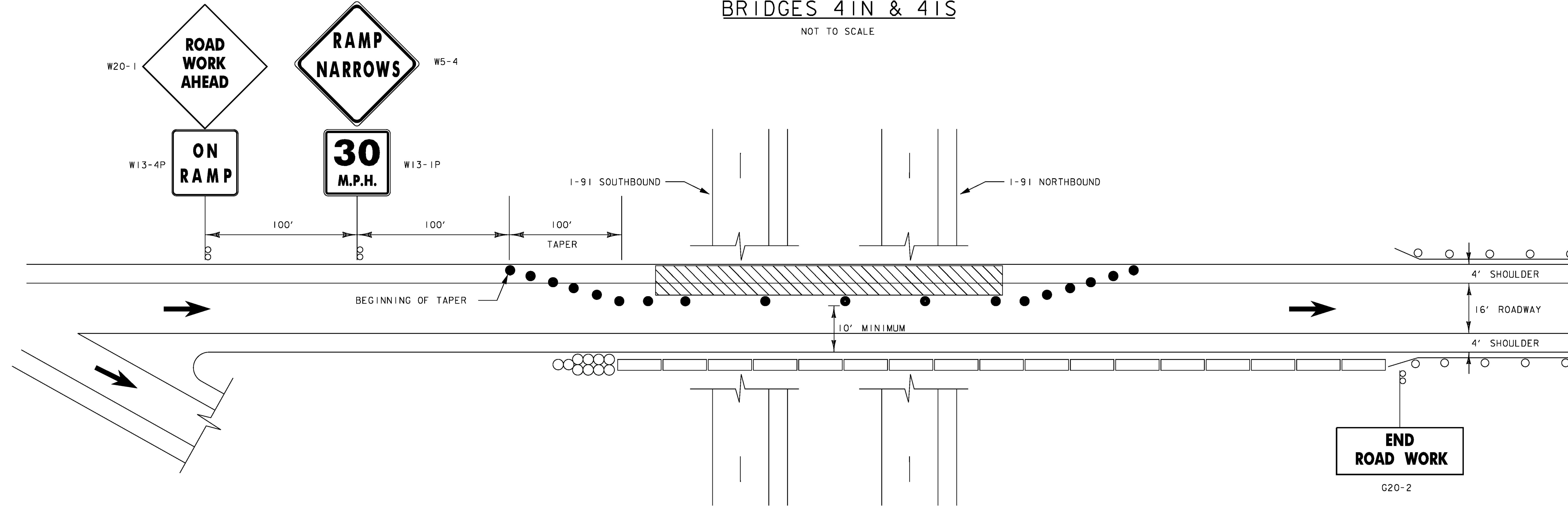
TRAFFIC CONTROL ON I-91 RAMP C, LANE SHIFT RIGHT BRIDGES 41N & 41S
