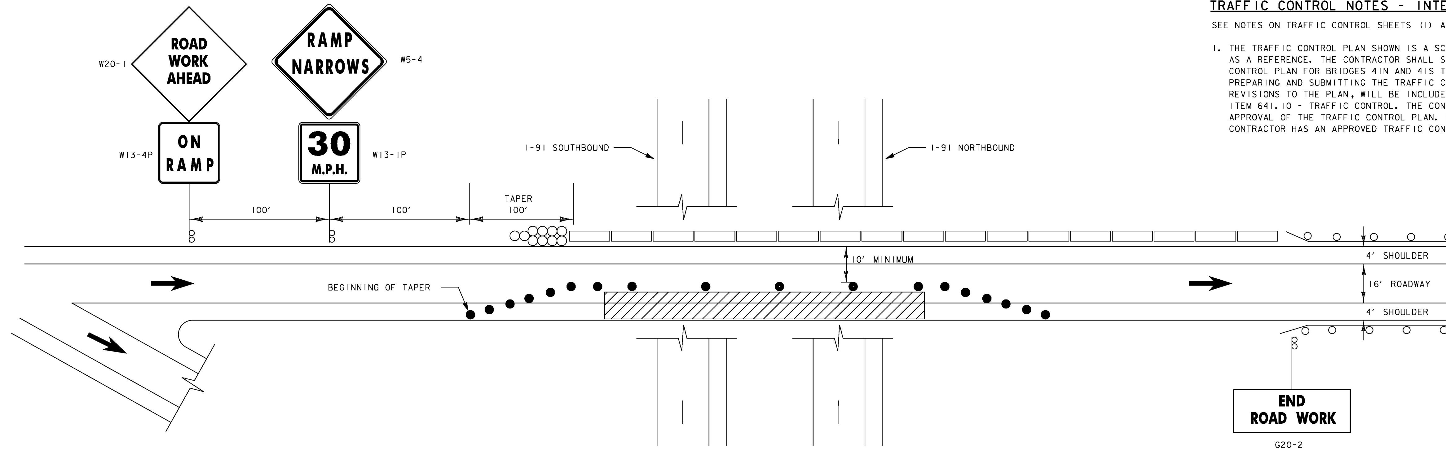
TRAFFIC CONTROL ON I-91 RAMP C, LANE SHIFT LEFT BRIDGES 41N & 41S
