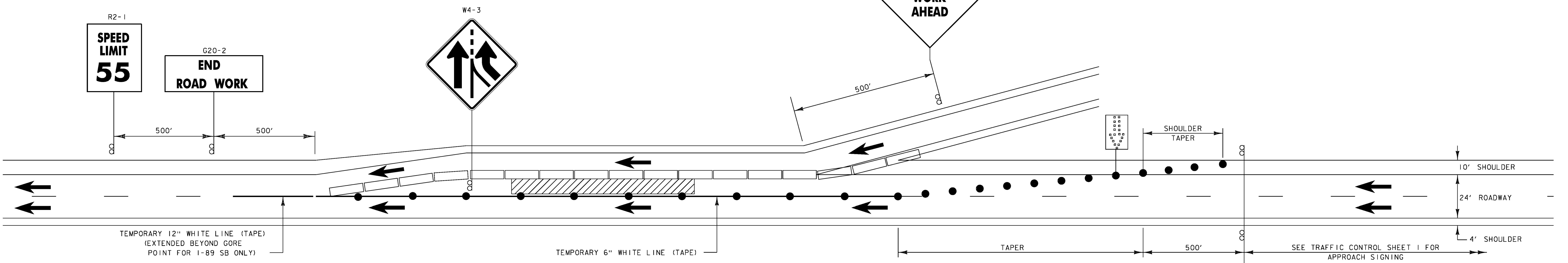
TRAFFIC CONTROL ON I-89, RIGHT LANE CLOSED BRIDGE 42 (SOUTHBOUND) NOT TO SCALE
