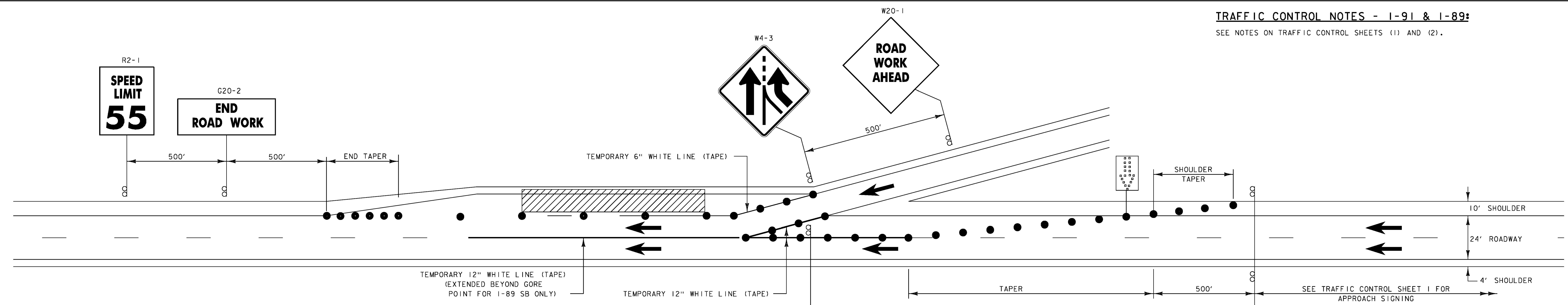
TRAFFIC CONTROL ON I-89, ACCEL LANE CLOSED BRIDGE 42 (SOUTHBOUND) NOT TO SCALE
