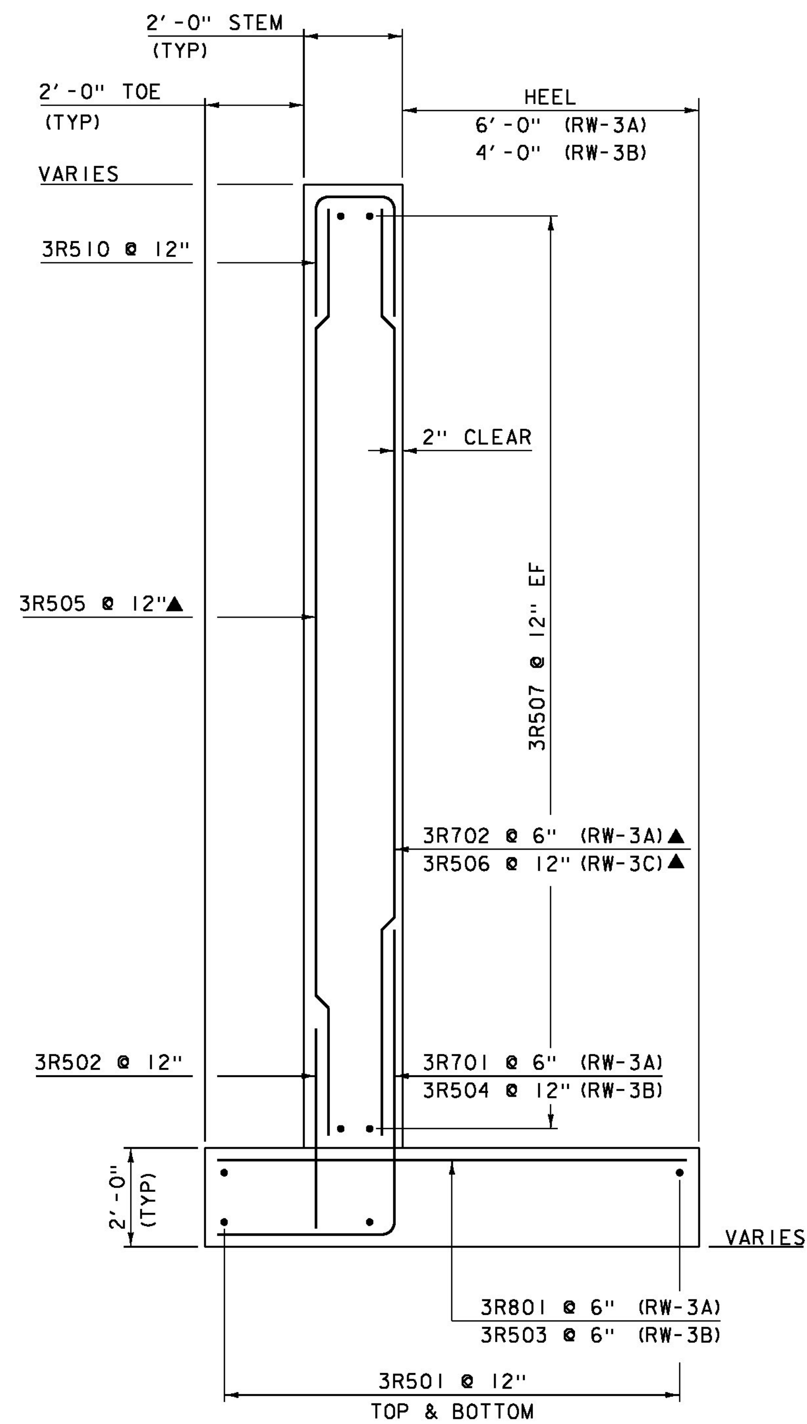
RETAINING WALL #3 TYPICAL
