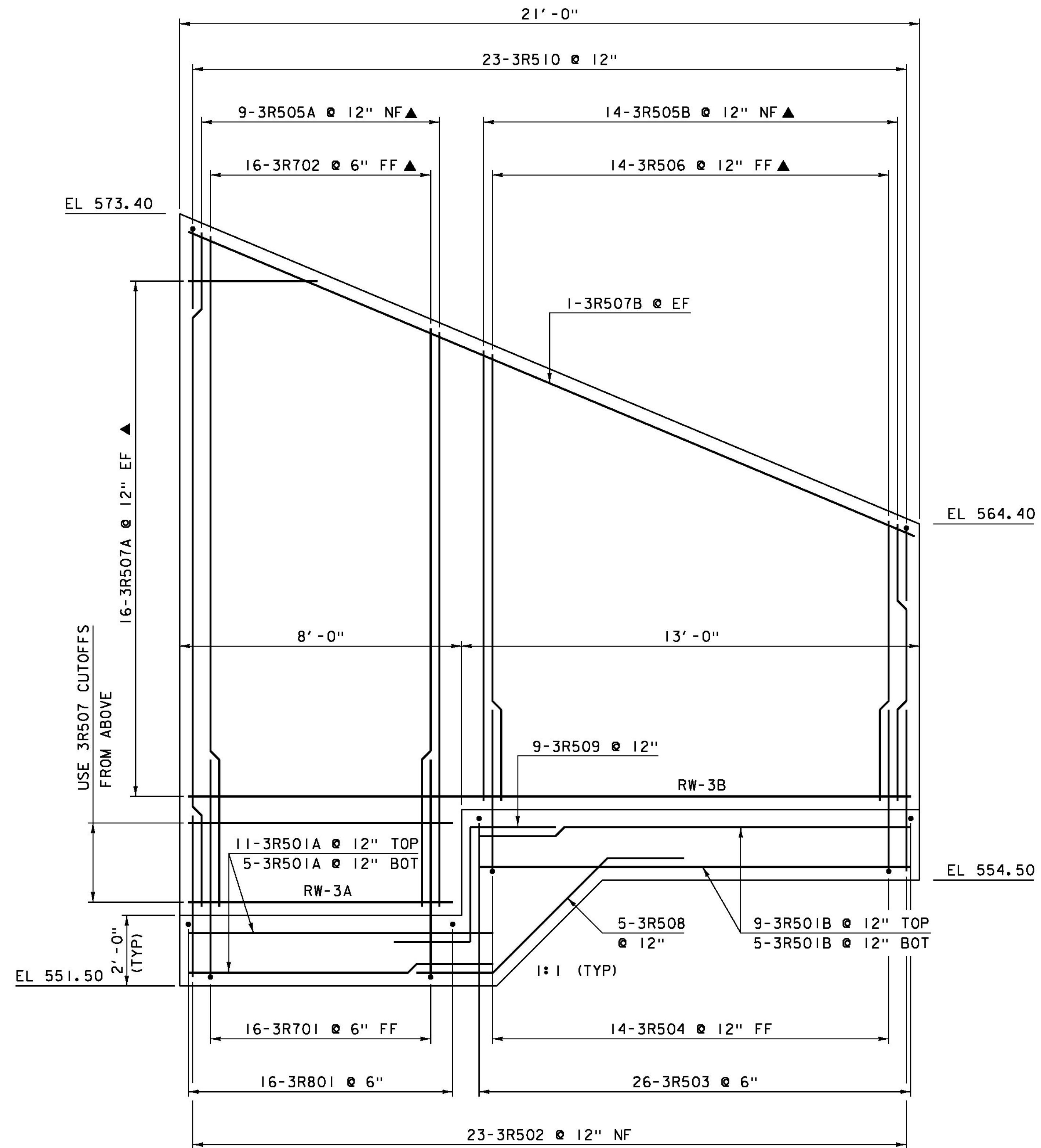
RETAINING WALL #3 ELEVATION
