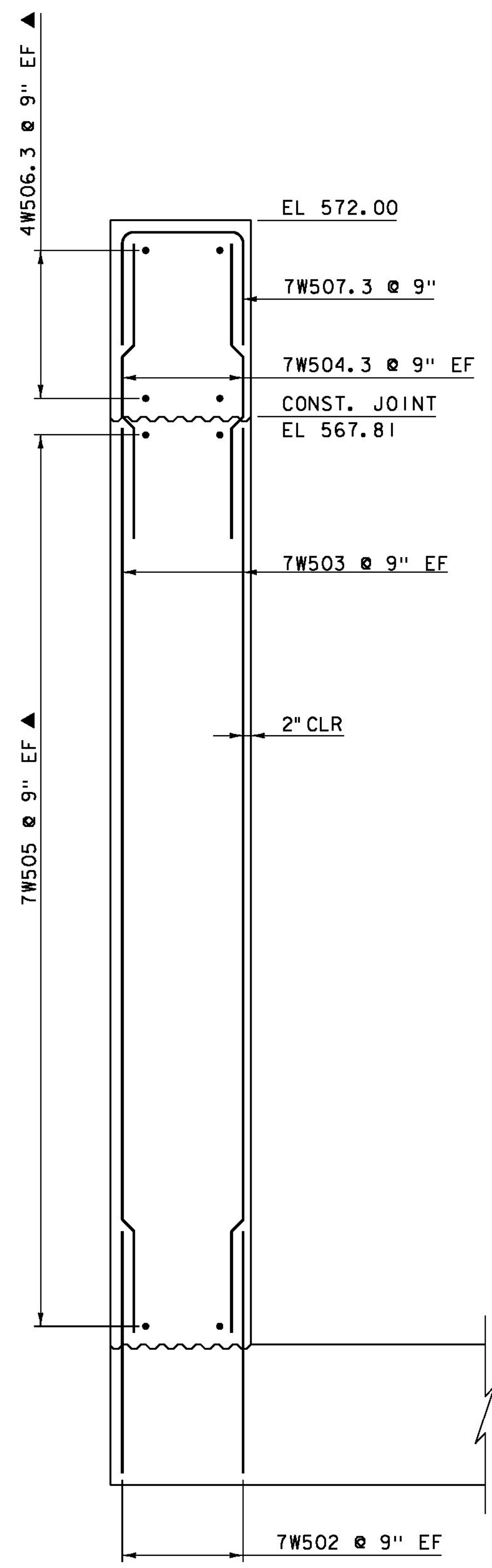
WINGWALL 7 TYPICAL SCALE: 1/2" = 1'-0"
