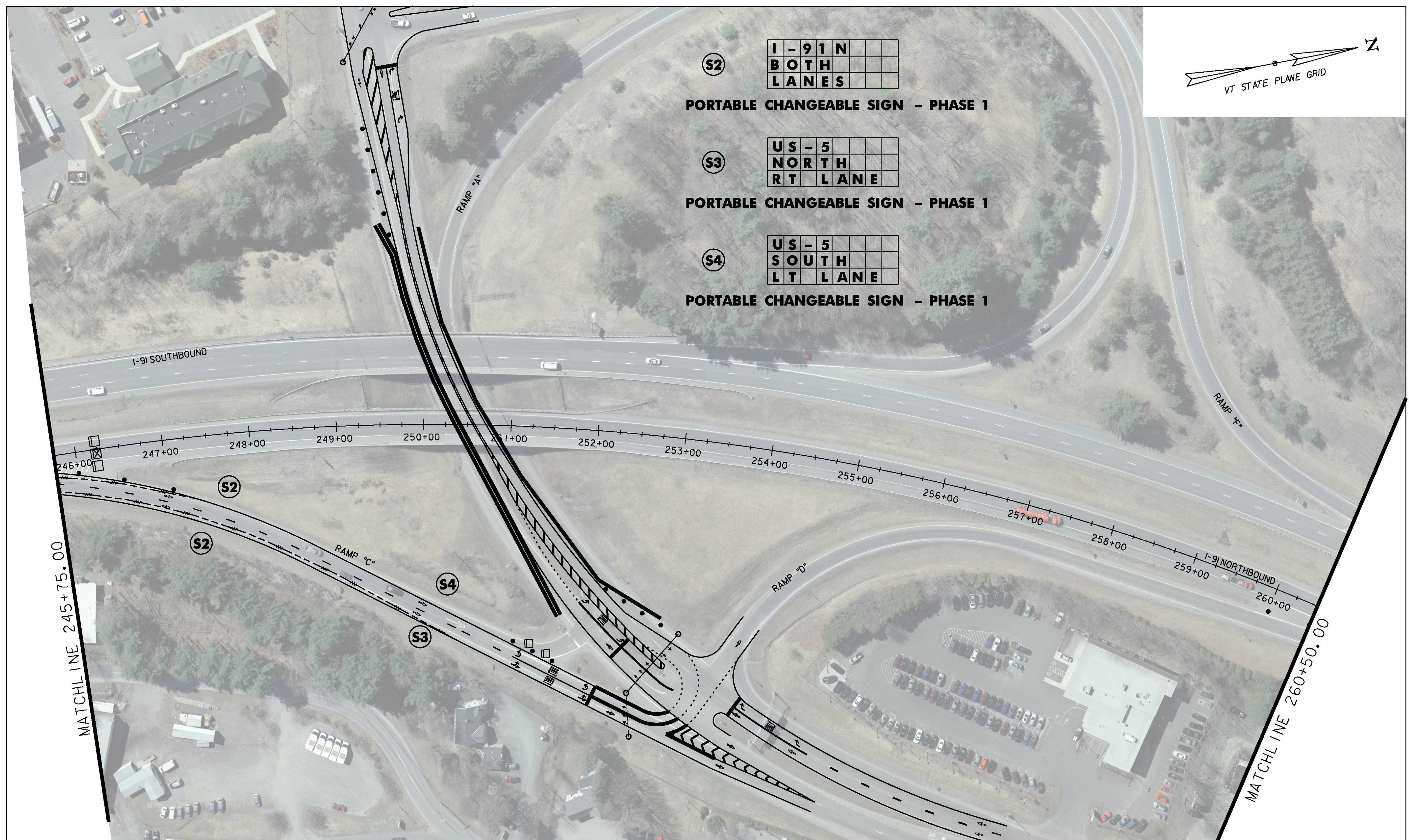
I-91 NB TRAFFIC CONTROL PLAN 4 (DURING BRIDGE CLOSURE)
